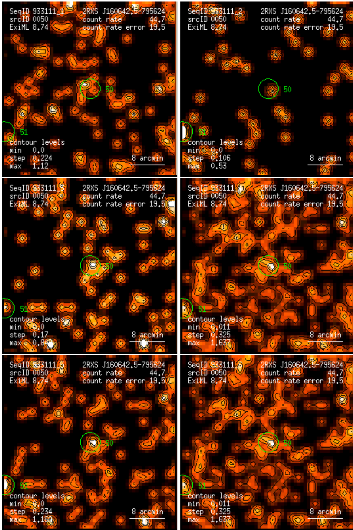
Figure 50: RASS 933111: detection 0050: band rate images, Gaussian filter: (1) PSPC channels 11 – 41, (2) 52 – 90, (3) 91 – 201, (4) 11 – 235, (5) 52 – 201, (6) 11 – 201. Broad band rates in counts/ks. Band rate contour levels in counts/ks/arcmin 2 .
