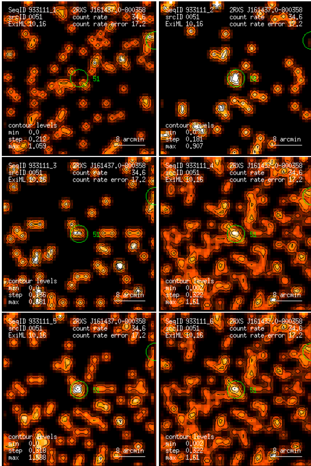
Figure 51: RASS 933111: detection 0051: band rate images, Gaussian filter: (1) PSPC channels 11 – 41, (2) 52 – 90, (3) 91 – 201, (4) 11 – 235, (5) 52 – 201, (6) 11 – 201. Broad band rates in counts/ks. Band rate contour levels in counts/ks/arcmin 2 .
