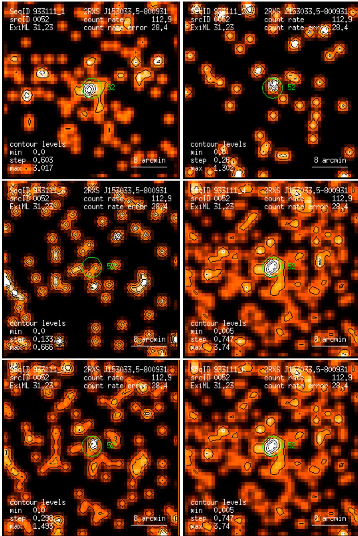
Figure 52: RASS 933111: detection 0052: band rate images, Gaussian filter: (1) PSPC channels 11 – 41, (2) 52 – 90, (3) 91 – 201, (4) 11 – 235, (5) 52 – 201, (6) 11 – 201. Broad band rates in counts/ks. Band rate contour levels in counts/ks/arcmin 2 .
