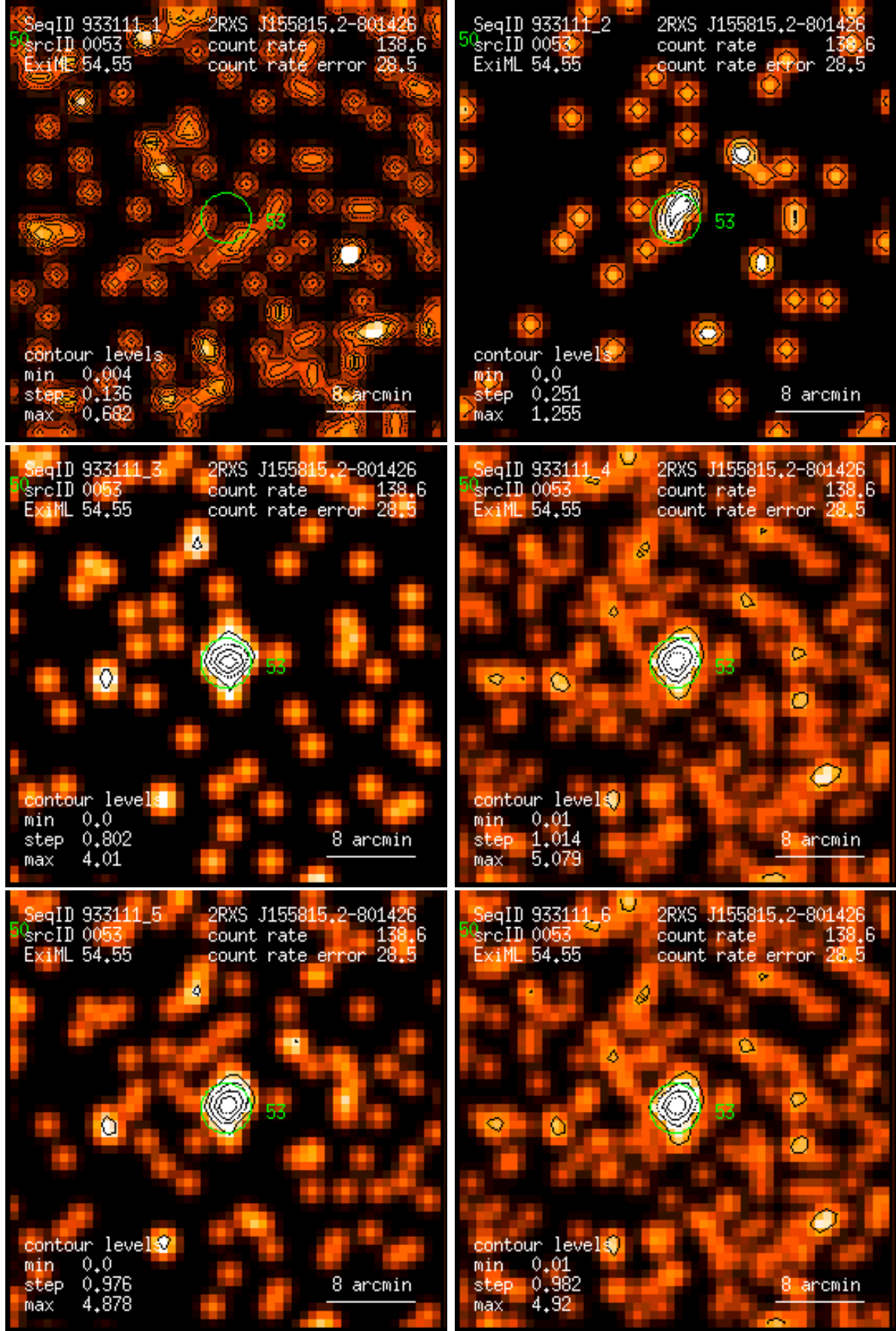
Figure 53: RASS 933111: detection 0053: band rate images, Gaussian filter: (1) PSPC channels 11 – 41, (2) 52 – 90, (3) 91 – 201, (4) 11 – 235, (5) 52 – 201, (6) 11 – 201. Broad band rates in counts/ks. Band rate contour levels in counts/ks/arcmin 2 .
