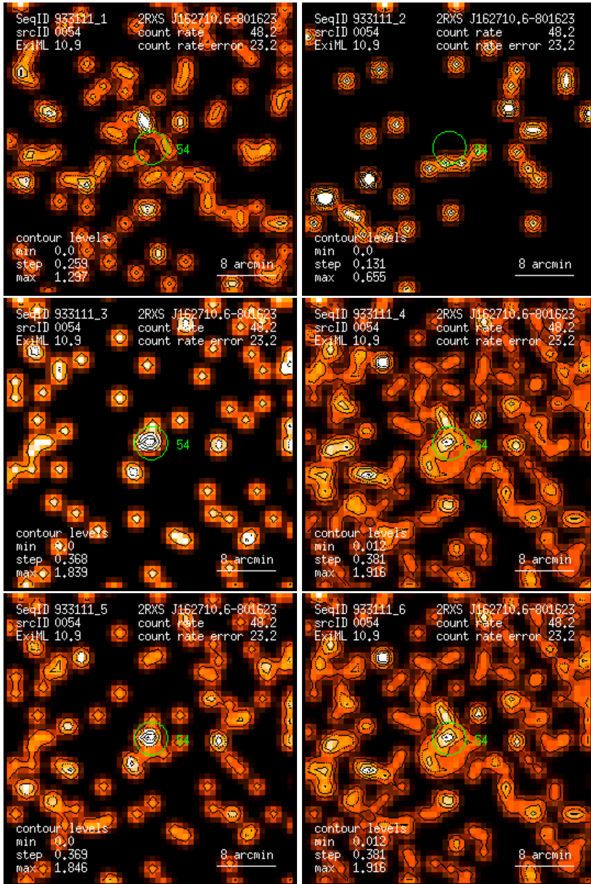
Figure 54: RASS 933111: detection 0054: band rate images, Gaussian filter: (1) PSPC channels 11 – 41, (2) 52 – 90, (3) 91 – 201, (4) 11 – 235, (5) 52 – 201, (6) 11 – 201. Broad band rates in counts/ks. Band rate contour levels in counts/ks/arcmin 2 .
