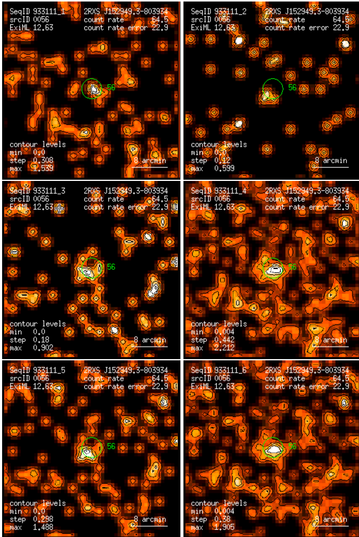
Figure 56: RASS 933111: detection 0056: band rate images, Gaussian filter: (1) PSPC channels 11 – 41, (2) 52 – 90, (3) 91 – 201, (4) 11 – 235, (5) 52 – 201, (6) 11 – 201. Broad band rates in counts/ks. Band rate contour levels in counts/ks/arcmin 2 .
