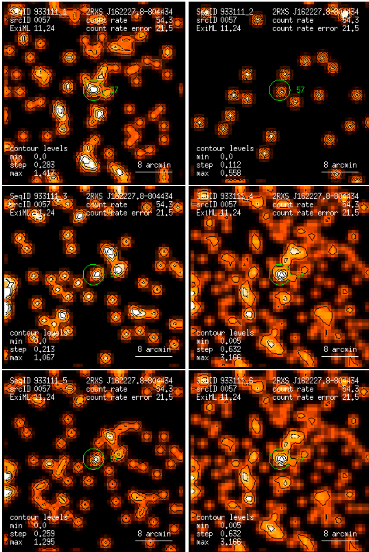
Figure 57: RASS 933111: detection 0057: band rate images, Gaussian filter: (1) PSPC channels 11 – 41, (2) 52 – 90, (3) 91 – 201, (4) 11 – 235, (5) 52 – 201, (6) 11 – 201. Broad band rates in counts/ks. Band rate contour levels in counts/ks/arcmin 2 .
