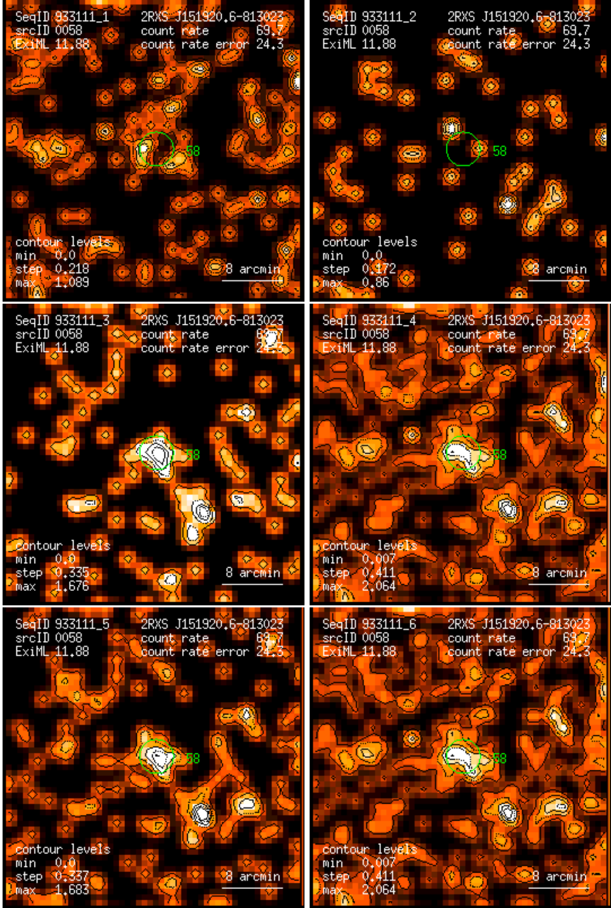
Figure 58: RASS 933111: detection 0058: band rate images, Gaussian filter: (1) PSPC channels 11 – 41, (2) 52 – 90, (3) 91 – 201, (4) 11 – 235, (5) 52 – 201, (6) 11 – 201. Broad band rates in counts/ks. Band rate contour levels in counts/ks/arcmin 2 .
