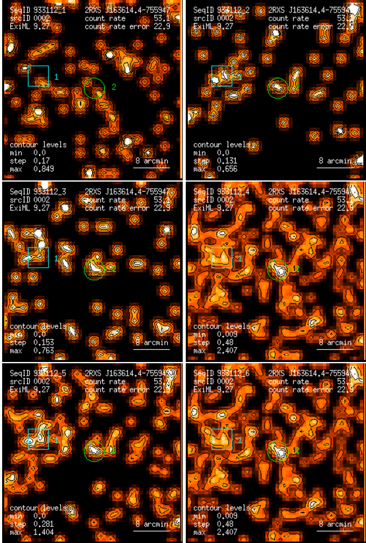
Figure 2: RASS 933112: detection 0002: band rate images, Gaussian filter: (1) PSPC channels 11 – 41, (2) 52 – 90, (3) 91 – 201, (4) 11 – 235, (5) 52 – 201, (6) 11 – 201. Broad band rates in counts/ks. Band rate contour levels in counts/ks/arcmin 2 .
