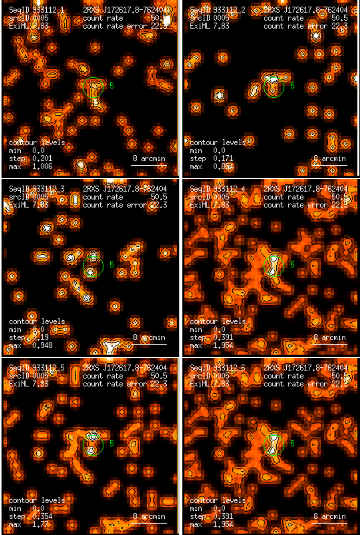
Figure 5: RASS 933112: detection 0005: band rate images, Gaussian filter: (1) PSPC channels 11 – 41, (2) 52 – 90, (3) 91 – 201, (4) 11 – 235, (5) 52 – 201, (6) 11 – 201. Broad band rates in counts/ks. Band rate contour levels in counts/ks/arcmin 2 .
