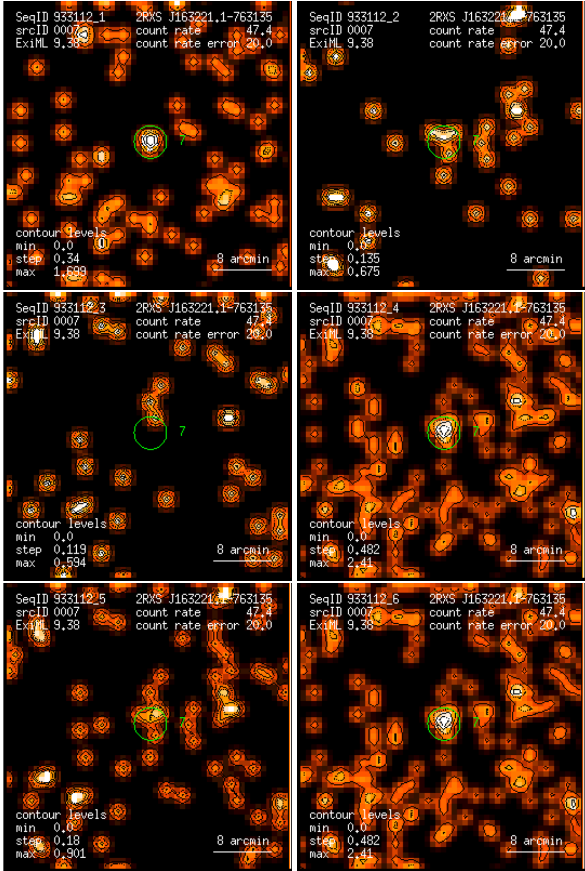
Figure 7: RASS 933112: detection 0007: band rate images, Gaussian filter: (1) PSPC channels 11 – 41, (2) 52 – 90, (3) 91 – 201, (4) 11 – 235, (5) 52 – 201, (6) 11 – 201. Broad band rates in counts/ks. Band rate contour levels in counts/ks/arcmin 2 .
