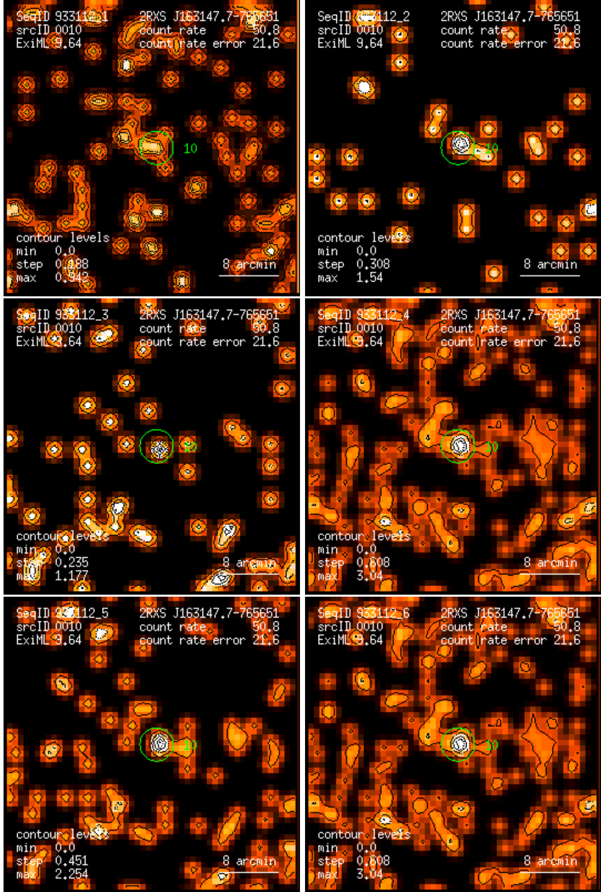
Figure 10: RASS 933112: detection 0010: band rate images, Gaussian filter: (1) PSPC channels 11 – 41, (2) 52 – 90, (3) 91 – 201, (4) 11 – 235, (5) 52 – 201, (6) 11 – 201. Broad band rates in counts/ks. Band rate contour levels in counts/ks/arcmin 2 .
