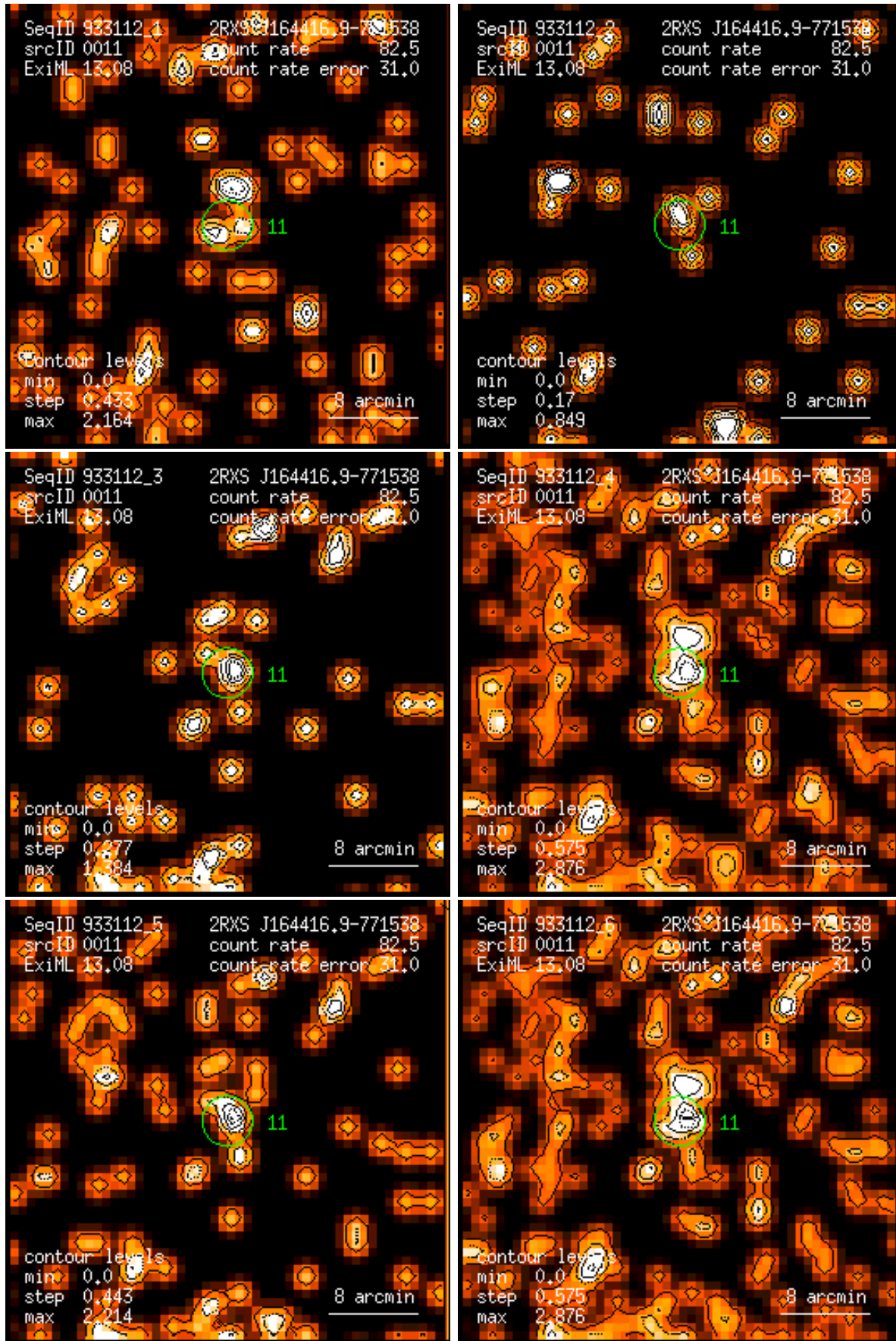
Figure 11: RASS 933112: detection 0011: band rate images, Gaussian filter: (1) PSPC channels 11 – 41, (2) 52 – 90, (3) 91 – 201, (4) 11 – 235, (5) 52 – 201, (6) 11 – 201. Broad band rates in counts/ks. Band rate contour levels in counts/ks/arcmin 2 .
