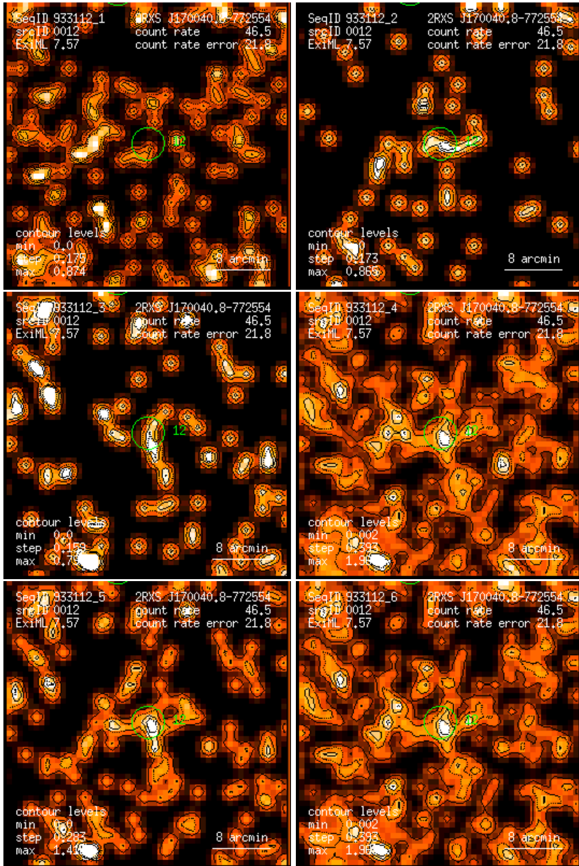
Figure 12: RASS 933112: detection 0012: band rate images, Gaussian filter: (1) PSPC channels 11 – 41, (2) 52 – 90, (3) 91 – 201, (4) 11 – 235, (5) 52 – 201, (6) 11 – 201. Broad band rates in counts/ks. Band rate contour levels in counts/ks/arcmin 2 .
