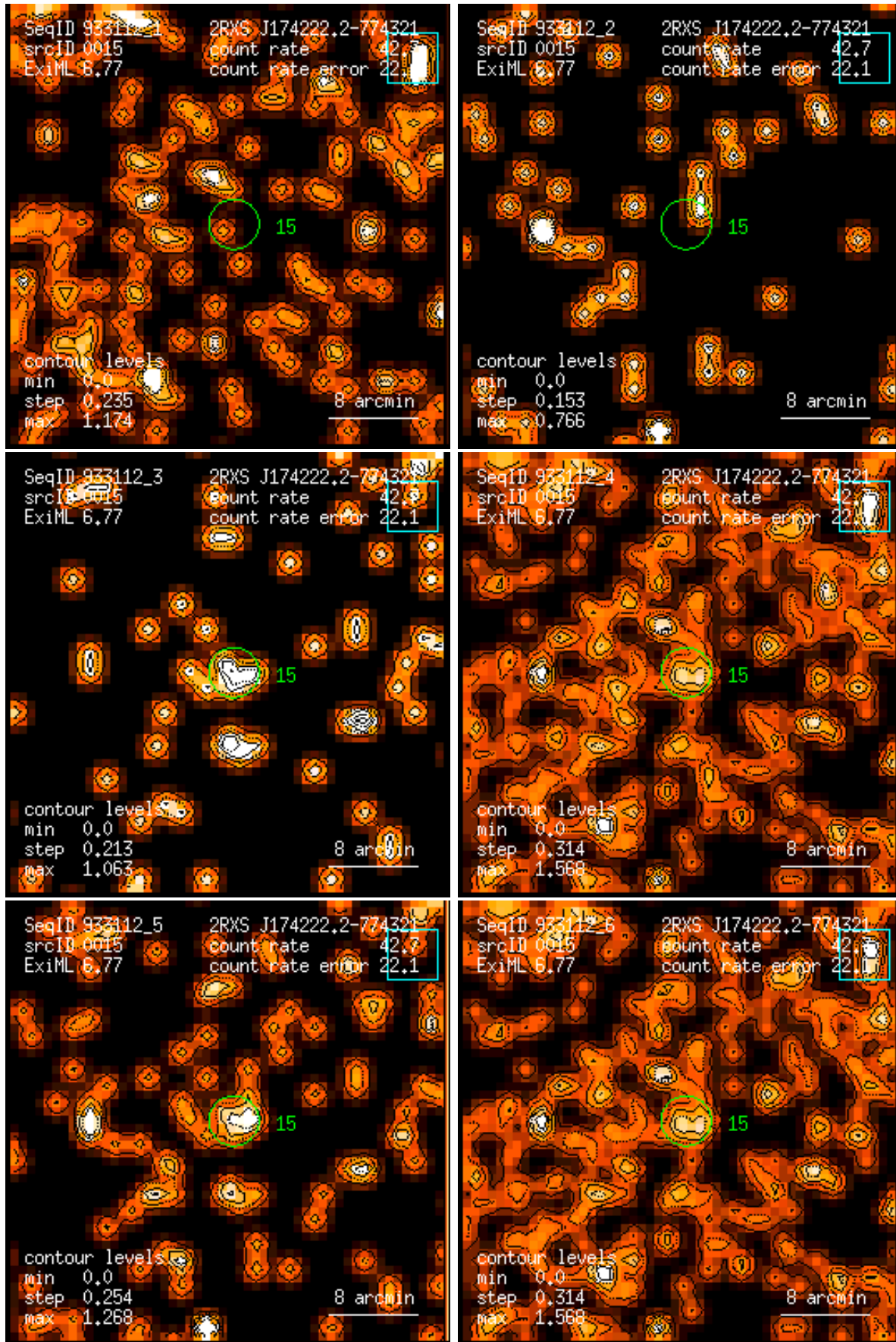
Figure 15: RASS 933112: detection 0015: band rate images, Gaussian filter: (1) PSPC channels 11 – 41, (2) 52 – 90, (3) 91 – 201, (4) 11 – 235, (5) 52 – 201, (6) 11 – 201. Broad band rates in counts/ks. Band rate contour levels in counts/ks/arcmin 2 .
