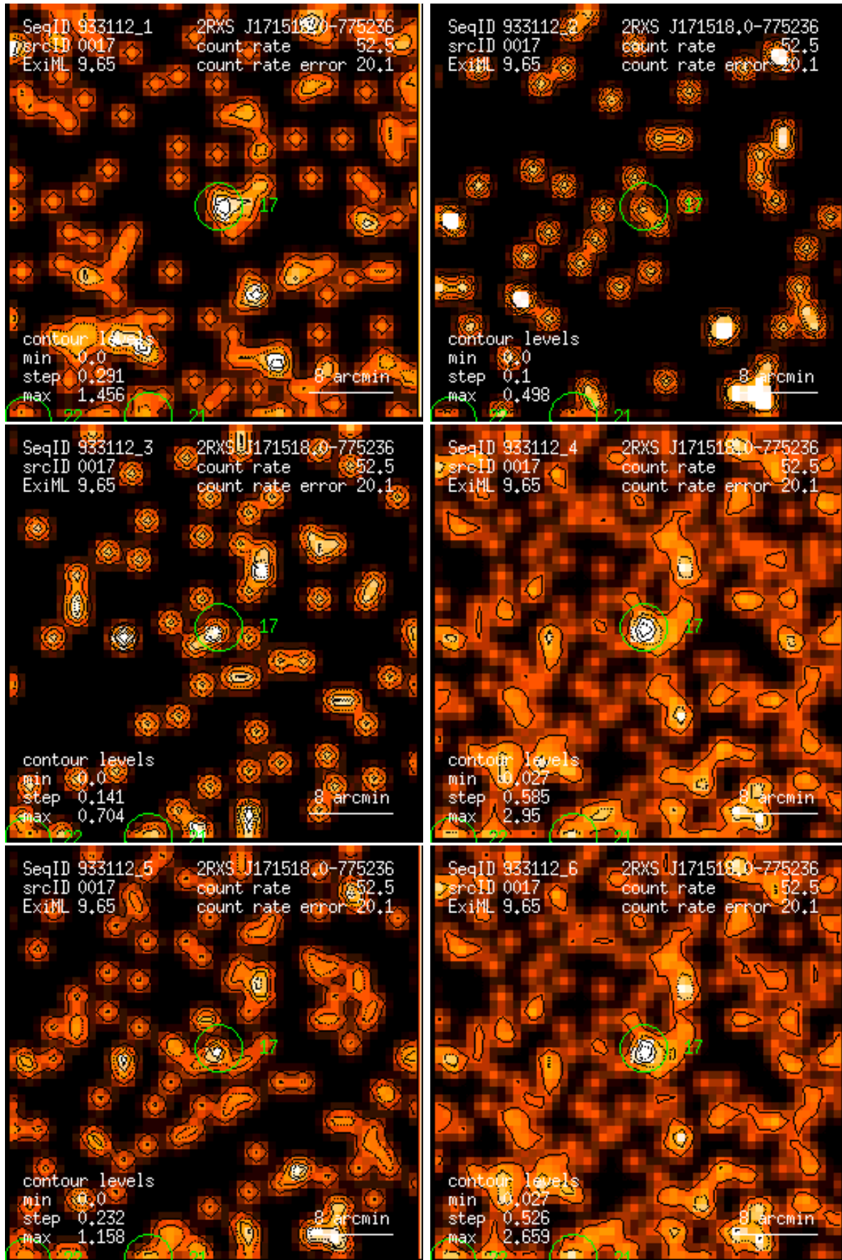
Figure 17: RASS 933112: detection 0017: band rate images, Gaussian filter: (1) PSPC channels 11 – 41, (2) 52 – 90, (3) 91 – 201, (4) 11 – 235, (5) 52 – 201, (6) 11 – 201. Broad band rates in counts/ks. Band rate contour levels in counts/ks/arcmin 2 .
