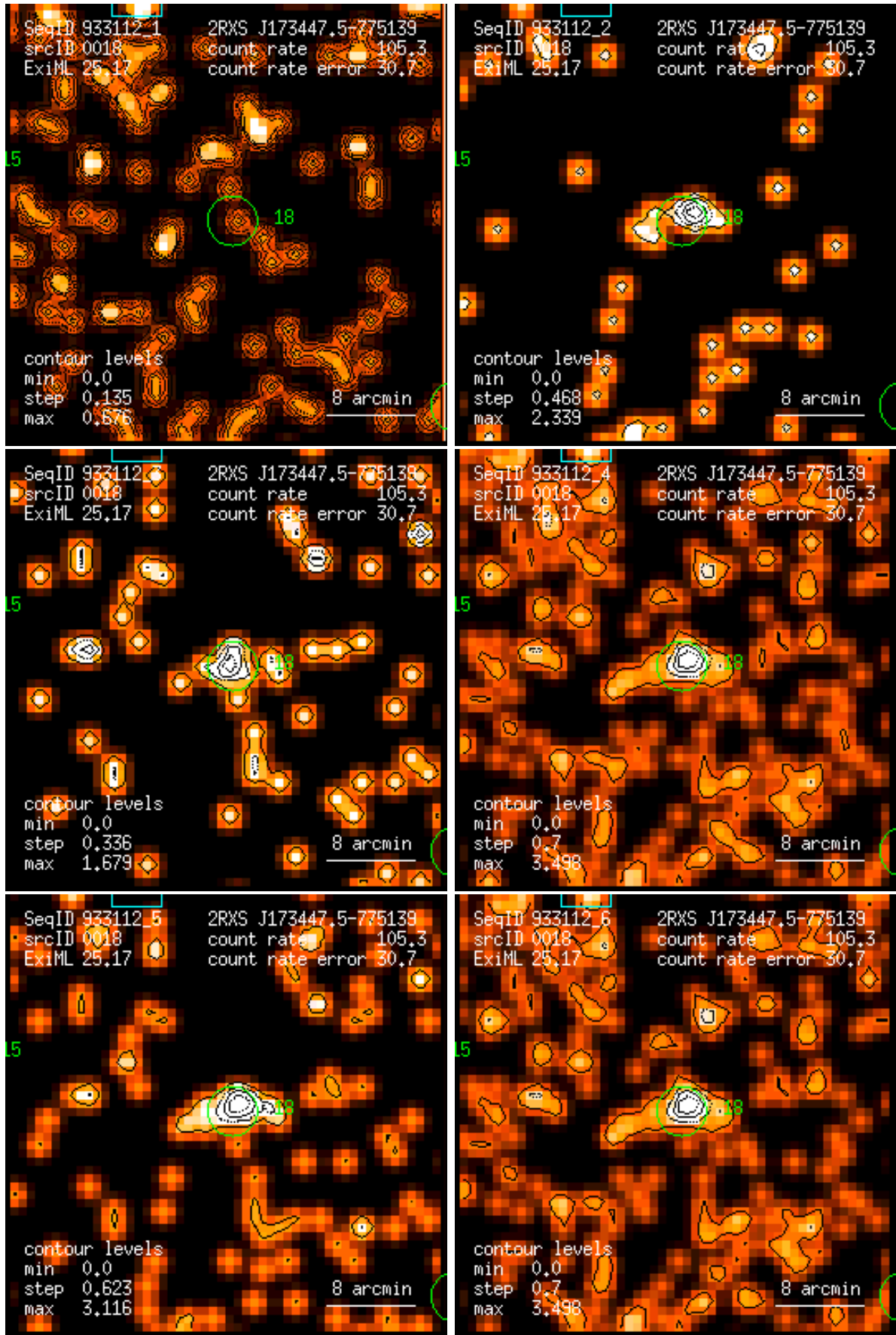
Figure 18: RASS 933112: detection 0018: band rate images, Gaussian filter: (1) PSPC channels 11 – 41, (2) 52 – 90, (3) 91 – 201, (4) 11 – 235, (5) 52 – 201, (6) 11 – 201. Broad band rates in counts/ks. Band rate contour levels in counts/ks/arcmin 2 .
