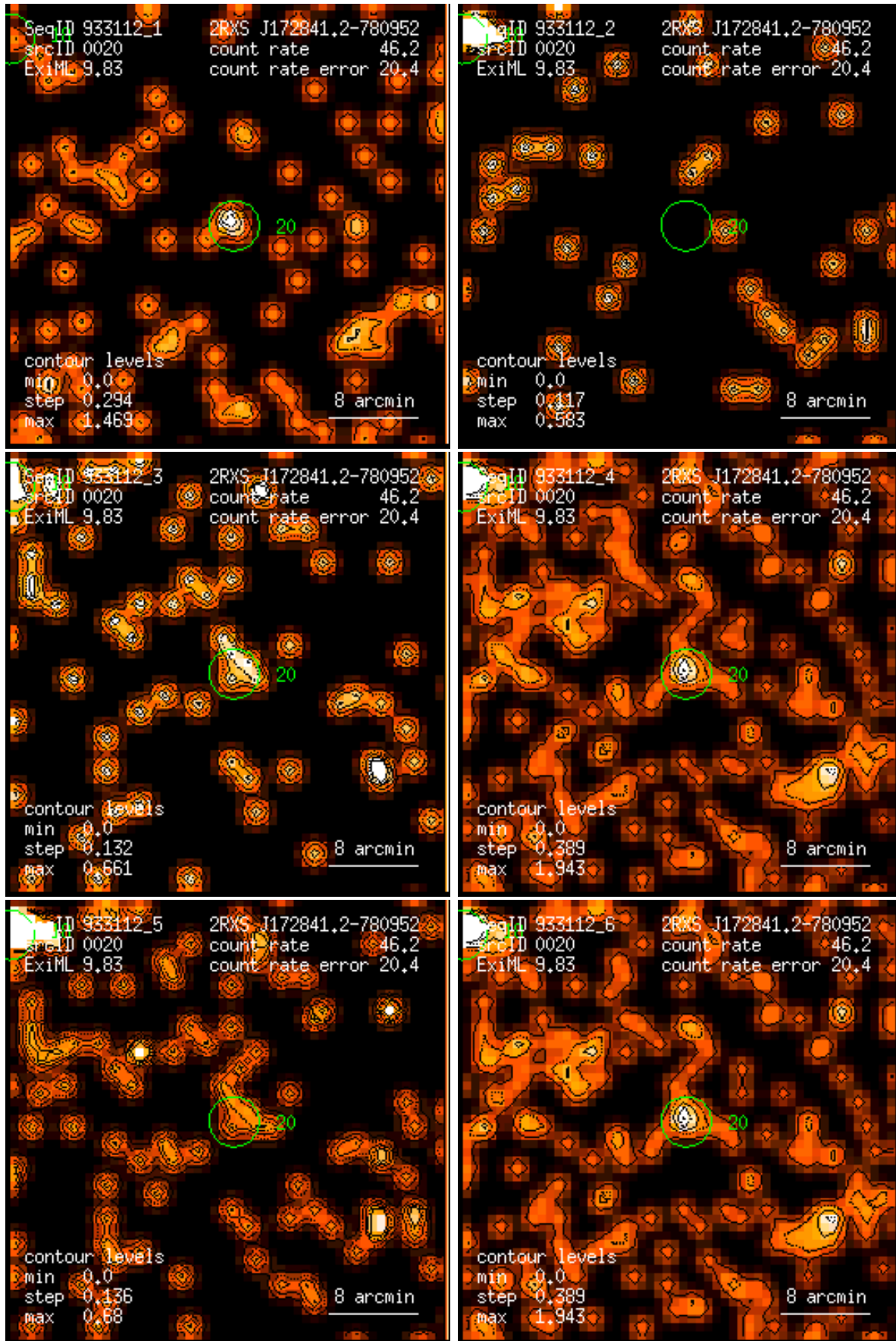
Figure 20: RASS 933112: detection 0020: band rate images, Gaussian filter: (1) PSPC channels 11 – 41, (2) 52 – 90, (3) 91 – 201, (4) 11 – 235, (5) 52 – 201, (6) 11 – 201. Broad band rates in counts/ks. Band rate contour levels in counts/ks/arcmin 2 .
