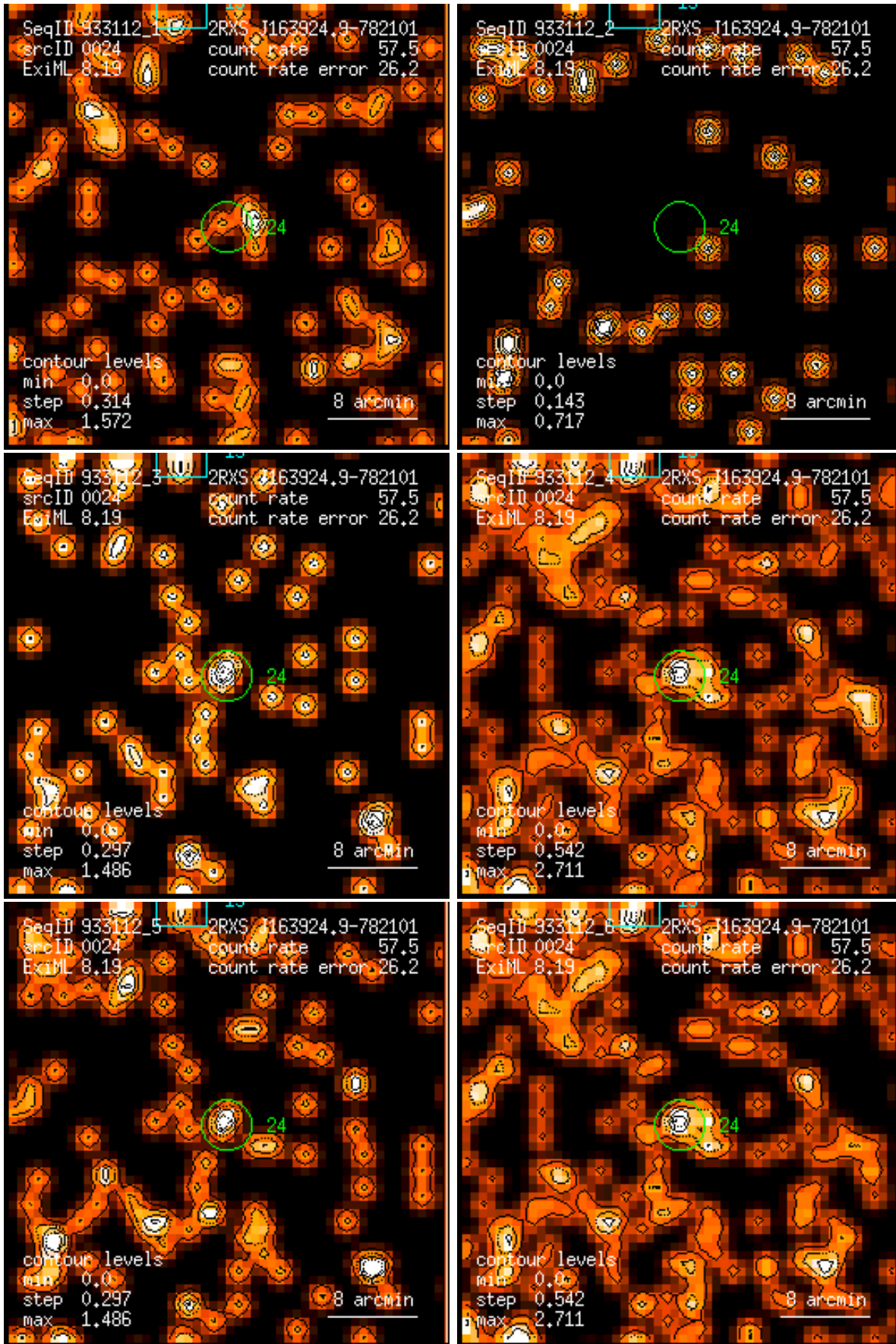
Figure 24: RASS 933112: detection 0024: band rate images, Gaussian filter: (1) PSPC channels 11 – 41, (2) 52 – 90, (3) 91 – 201, (4) 11 – 235, (5) 52 – 201, (6) 11 – 201. Broad band rates in counts/ks. Band rate contour levels in counts/ks/arcmin 2 .
