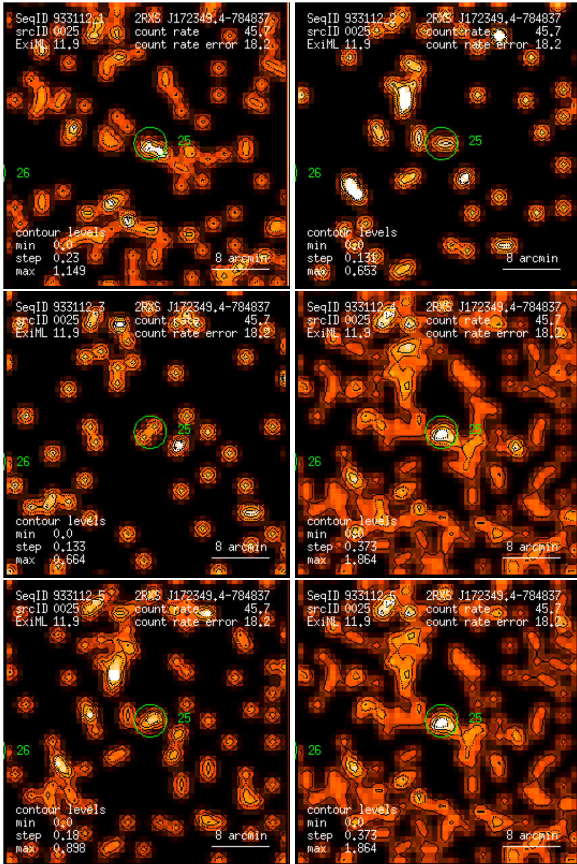
Figure 25: RASS 933112: detection 0025: band rate images, Gaussian filter: (1) PSPC channels 11 – 41, (2) 52 – 90, (3) 91 – 201, (4) 11 – 235, (5) 52 – 201, (6) 11 – 201. Broad band rates in counts/ks. Band rate contour levels in counts/ks/arcmin 2 .
