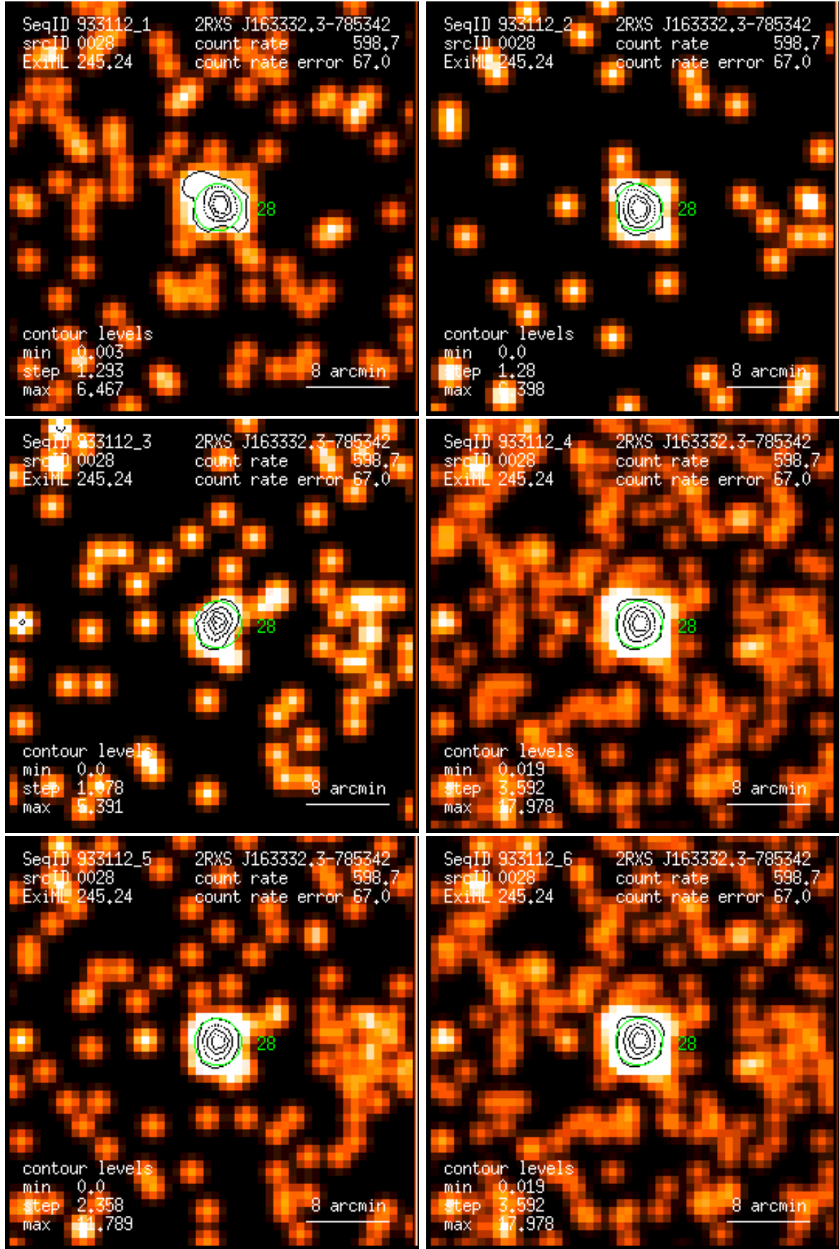
Figure 28: RASS 933112: detection 0028: band rate images, Gaussian filter: (1) PSPC channels 11 – 41, (2) 52 – 90, (3) 91 – 201, (4) 11 – 235, (5) 52 – 201, (6) 11 – 201. Broad band rates in counts/ks. Band rate contour levels in counts/ks/arcmin 2 .
