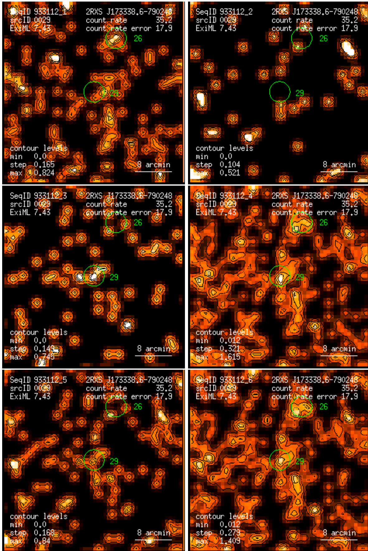
Figure 29: RASS 933112: detection 0029: band rate images, Gaussian filter: (1) PSPC channels 11 – 41, (2) 52 – 90, (3) 91 – 201, (4) 11 – 235, (5) 52 – 201, (6) 11 – 201. Broad band rates in counts/ks. Band rate contour levels in counts/ks/arcmin 2 .
