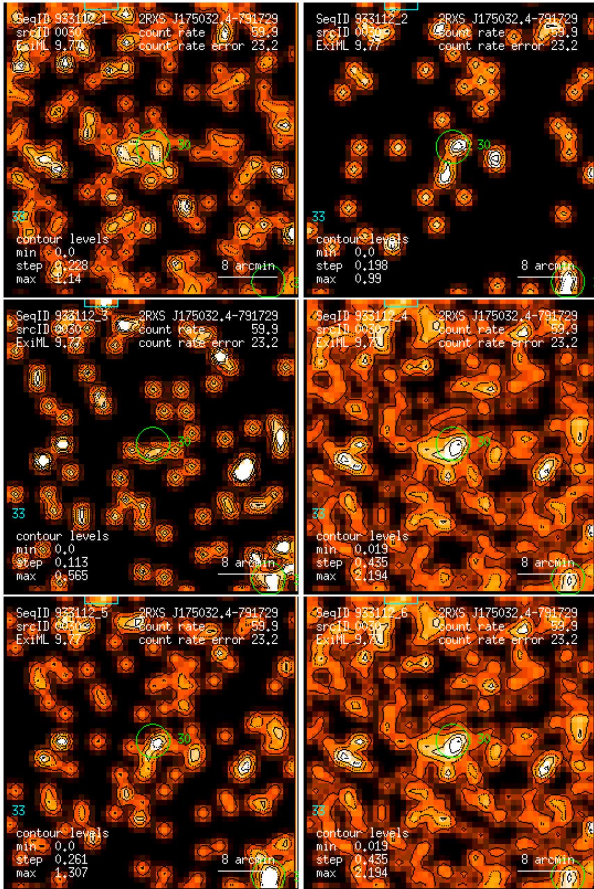
Figure 30: RASS 933112: detection 0030: band rate images, Gaussian filter: (1) PSPC channels 11 – 41, (2) 52 – 90, (3) 91 – 201, (4) 11 – 235, (5) 52 – 201, (6) 11 – 201. Broad band rates in counts/ks. Band rate contour levels in counts/ks/arcmin 2 .
