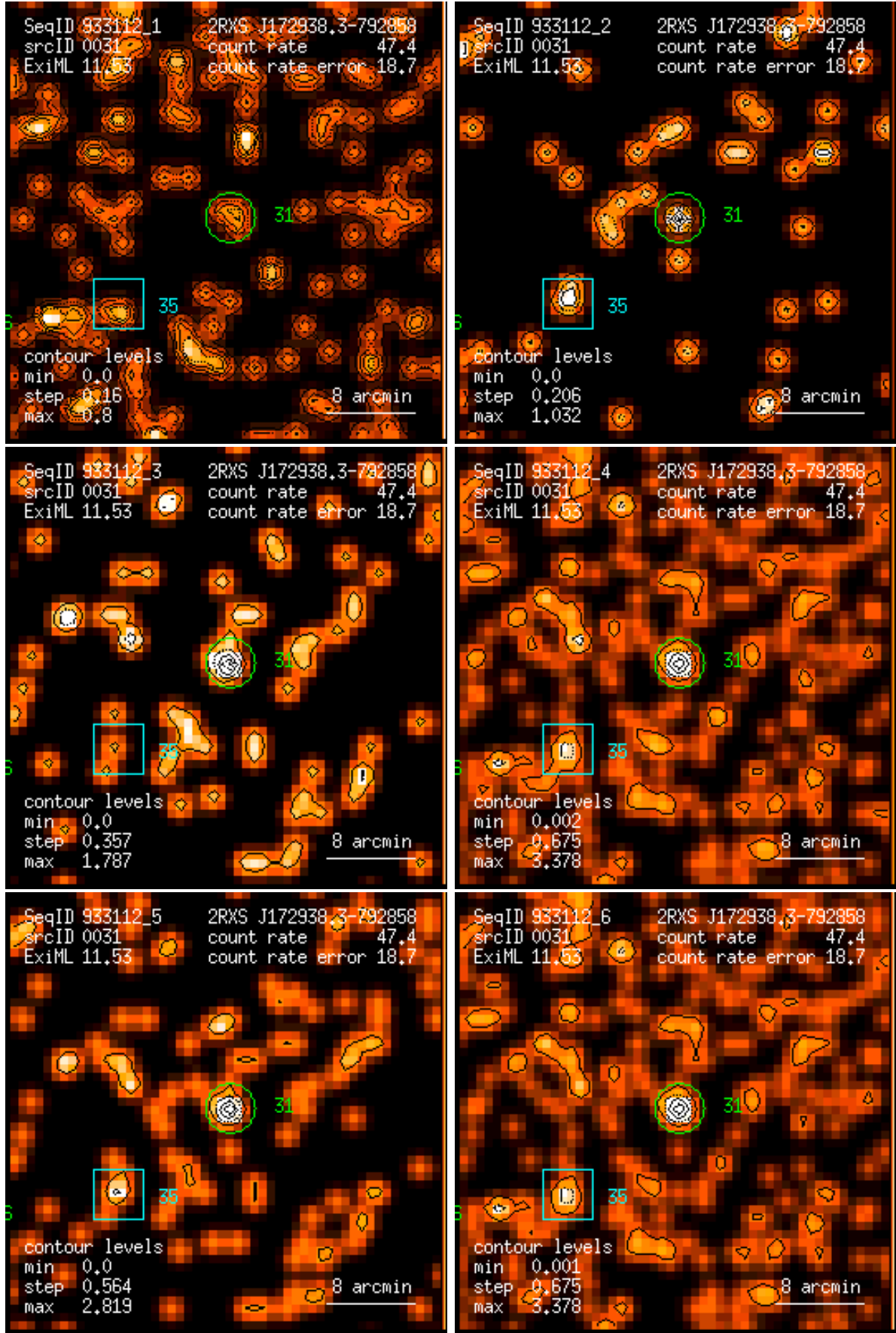
Figure 31: RASS 933112: detection 0031: band rate images, Gaussian filter: (1) PSPC channels 11 – 41, (2) 52 – 90, (3) 91 – 201, (4) 11 – 235, (5) 52 – 201, (6) 11 – 201. Broad band rates in counts/ks. Band rate contour levels in counts/ks/arcmin 2 .
