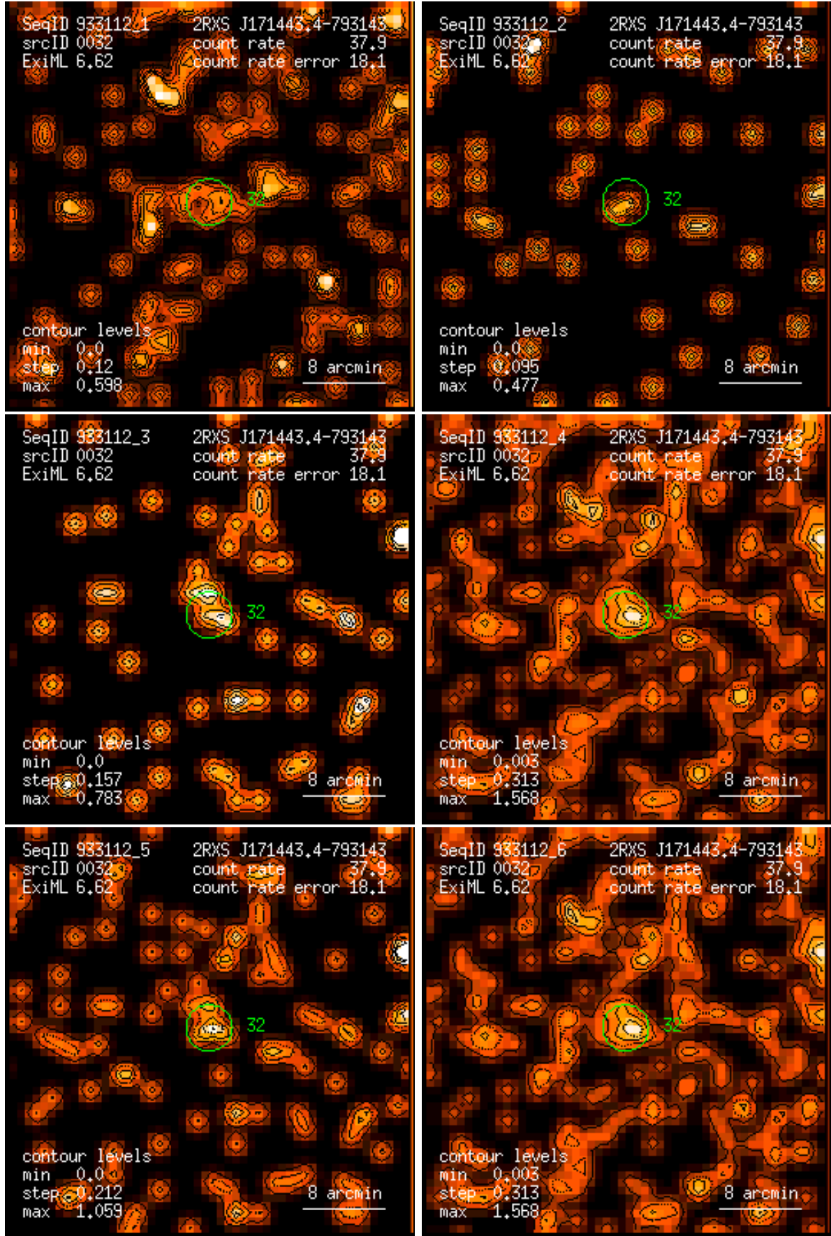
Figure 32: RASS 933112: detection 0032: band rate images, Gaussian filter: (1) PSPC channels 11 – 41, (2) 52 – 90, (3) 91 – 201, (4) 11 – 235, (5) 52 – 201, (6) 11 – 201. Broad band rates in counts/ks. Band rate contour levels in counts/ks/arcmin 2 .
