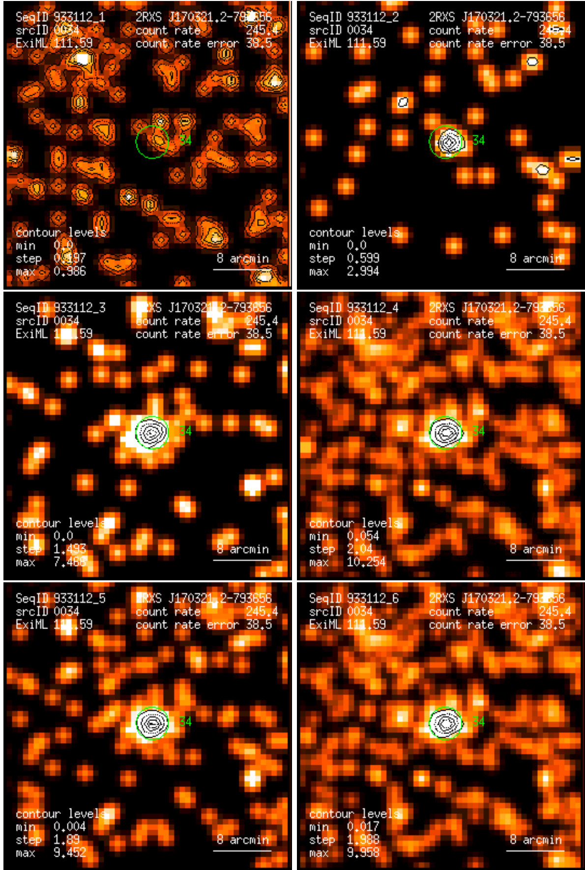
Figure 34: RASS 933112: detection 0034: band rate images, Gaussian filter: (1) PSPC channels 11 – 41, (2) 52 – 90, (3) 91 – 201, (4) 11 – 235, (5) 52 – 201, (6) 11 – 201. Broad band rates in counts/ks. Band rate contour levels in counts/ks/arcmin 2 .
