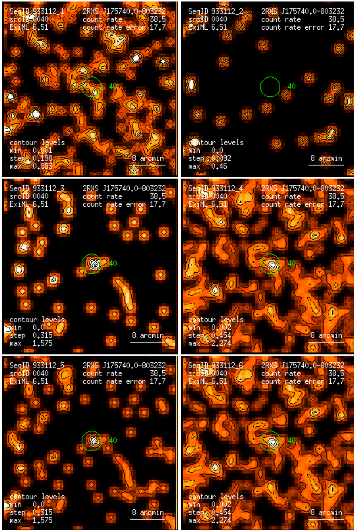
Figure 40: RASS 933112: detection 0040: band rate images, Gaussian filter: (1) PSPC channels 11 – 41, (2) 52 – 90, (3) 91 – 201, (4) 11 – 235, (5) 52 – 201, (6) 11 – 201. Broad band rates in counts/ks. Band rate contour levels in counts/ks/arcmin 2 .
