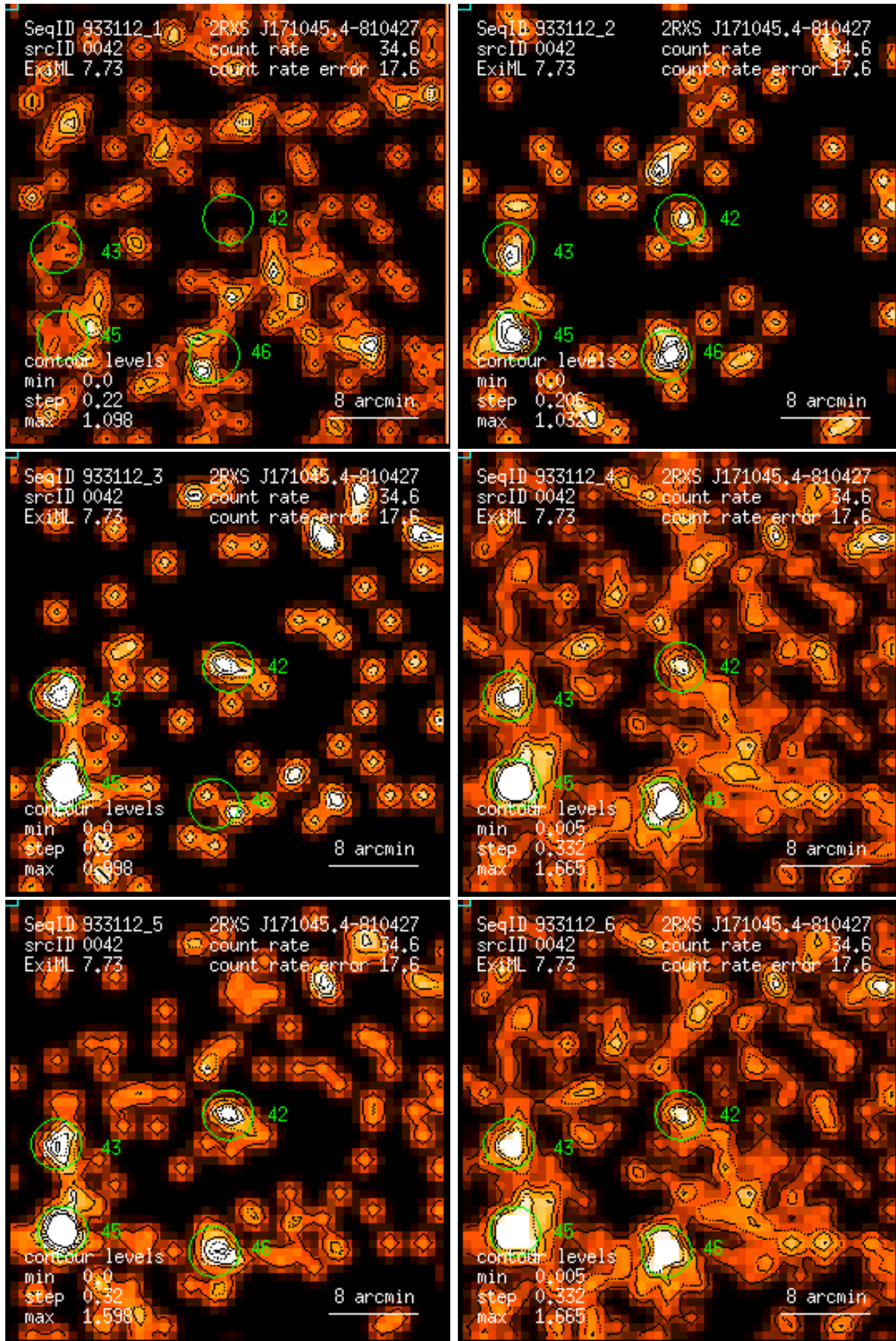
Figure 42: RASS 933112: detection 0042: band rate images, Gaussian filter: (1) PSPC channels 11 – 41, (2) 52 – 90, (3) 91 – 201, (4) 11 – 235, (5) 52 – 201, (6) 11 – 201. Broad band rates in counts/ks. Band rate contour levels in counts/ks/arcmin 2 .
