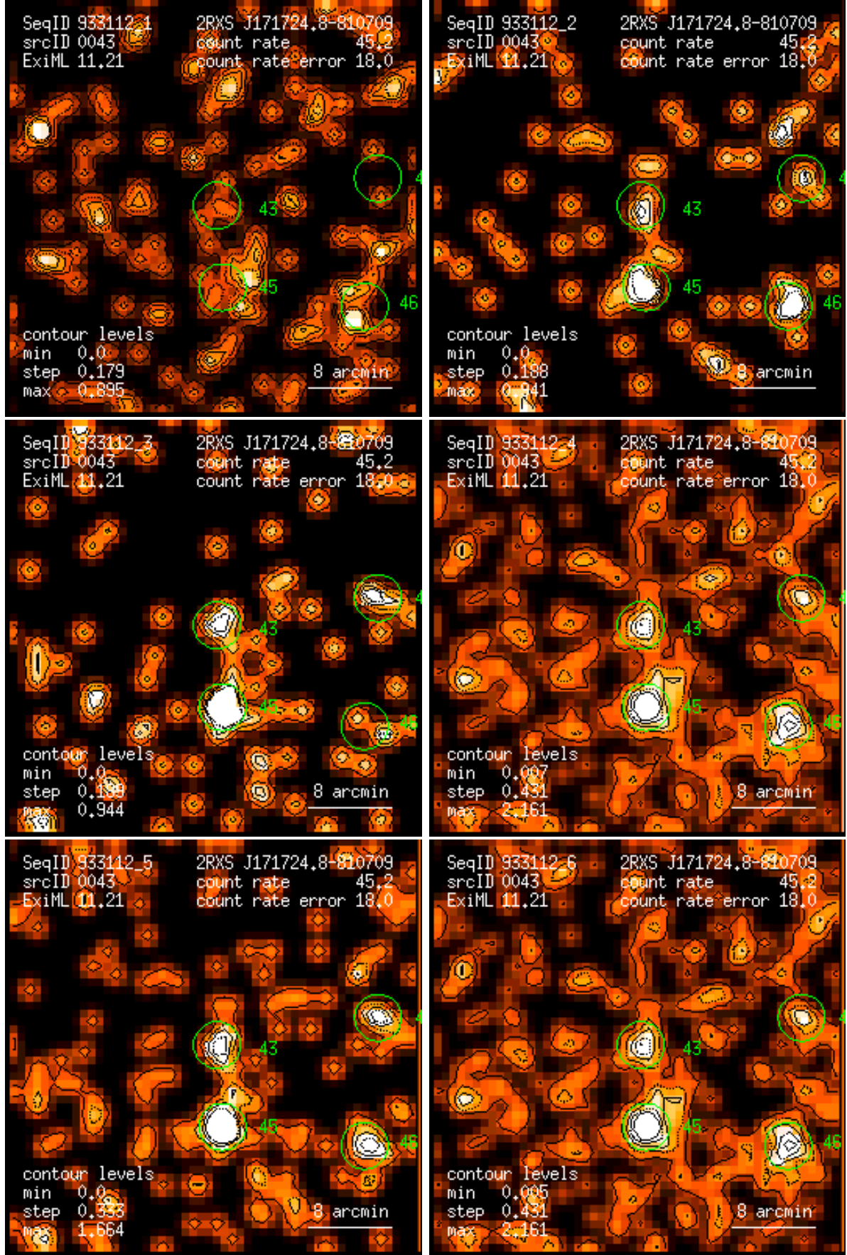
Figure 43: RASS 933112: detection 0043: band rate images, Gaussian filter: (1) PSPC channels 11 – 41, (2) 52 – 90, (3) 91 – 201, (4) 11 – 235, (5) 52 – 201, (6) 11 – 201. Broad band rates in counts/ks. Band rate contour levels in counts/ks/arcmin 2 .
