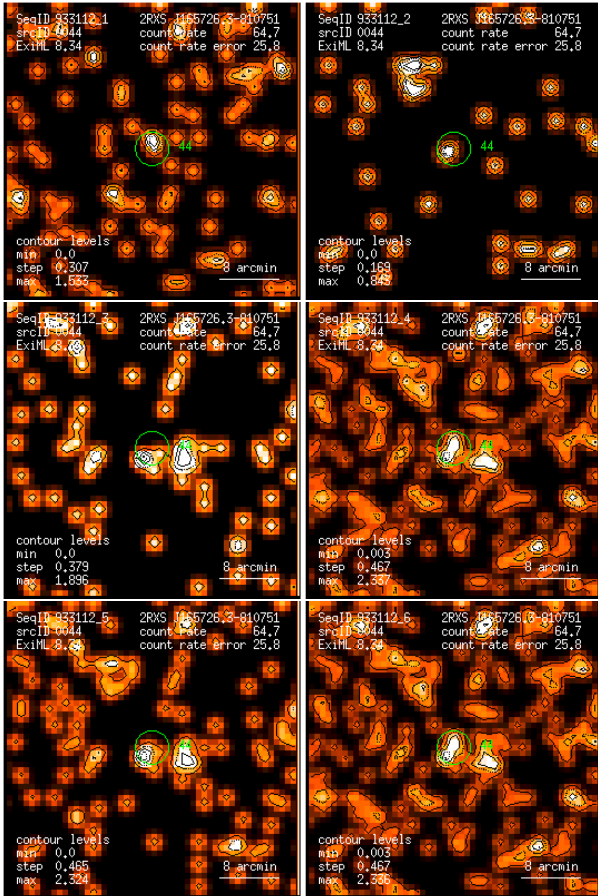
Figure 44: RASS 933112: detection 0044: band rate images, Gaussian filter: (1) PSPC channels 11 – 41, (2) 52 – 90, (3) 91 – 201, (4) 11 – 235, (5) 52 – 201, (6) 11 – 201. Broad band rates in counts/ks. Band rate contour levels in counts/ks/arcmin 2 .
