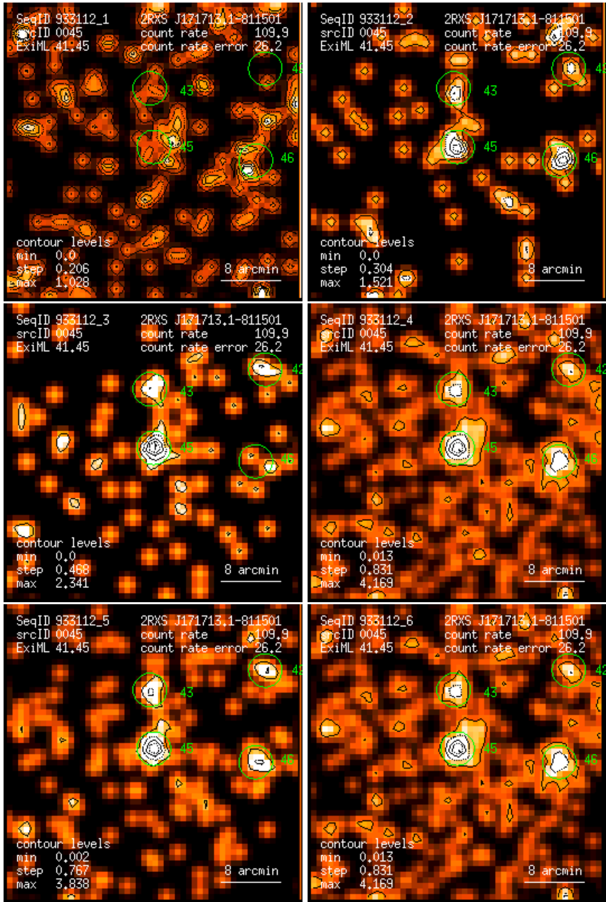
Figure 45: RASS 933112: detection 0045: band rate images, Gaussian filter: (1) PSPC channels 11 – 41, (2) 52 – 90, (3) 91 – 201, (4) 11 – 235, (5) 52 – 201, (6) 11 – 201. Broad band rates in counts/ks. Band rate contour levels in counts/ks/arcmin 2 .
