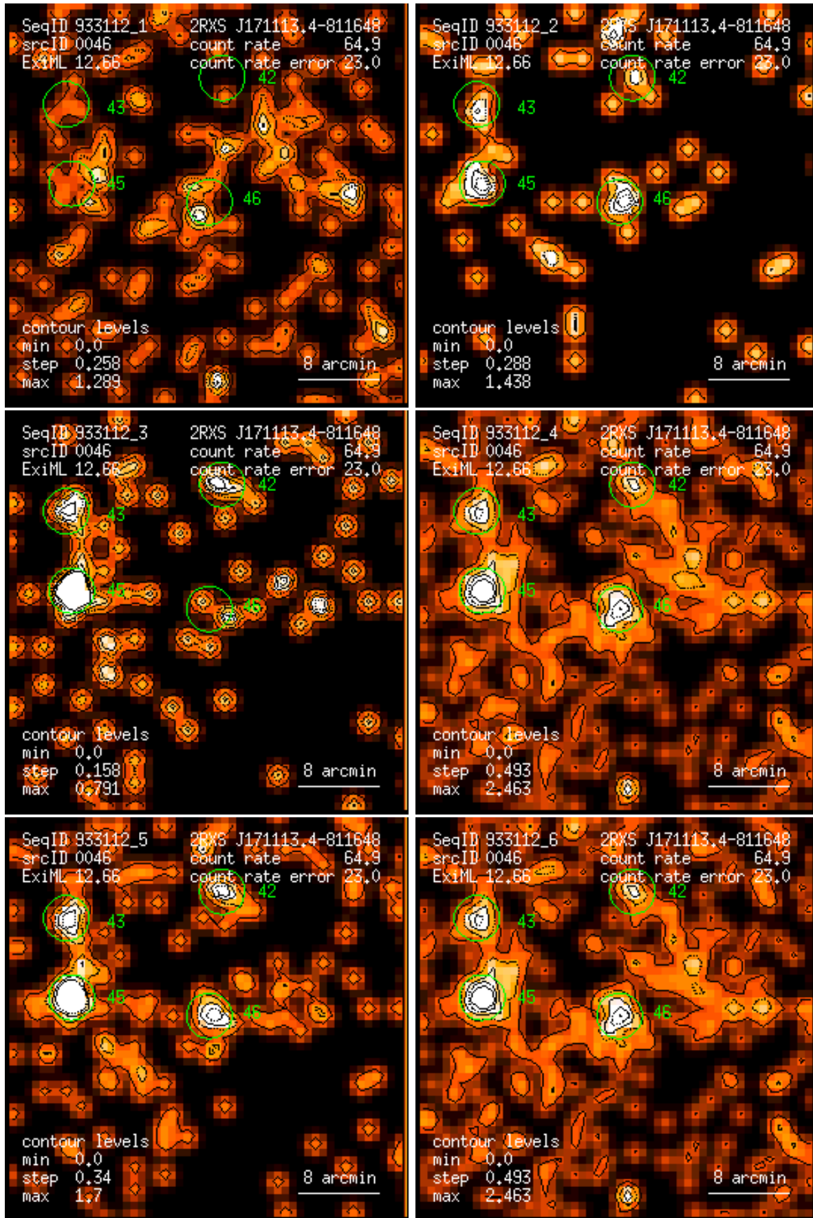
Figure 46: RASS 933112: detection 0046: band rate images, Gaussian filter: (1) PSPC channels 11 – 41, (2) 52 – 90, (3) 91 – 201, (4) 11 – 235, (5) 52 – 201, (6) 11 – 201. Broad band rates in counts/ks. Band rate contour levels in counts/ks/arcmin 2 .
