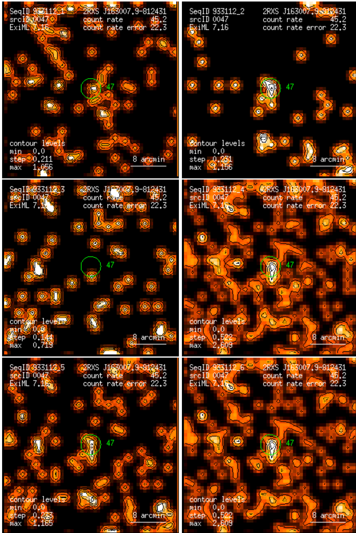
Figure 47: RASS 933112: detection 0047: band rate images, Gaussian filter: (1) PSPC channels 11 – 41, (2) 52 – 90, (3) 91 – 201, (4) 11 – 235, (5) 52 – 201, (6) 11 – 201. Broad band rates in counts/ks. Band rate contour levels in counts/ks/arcmin 2 .
