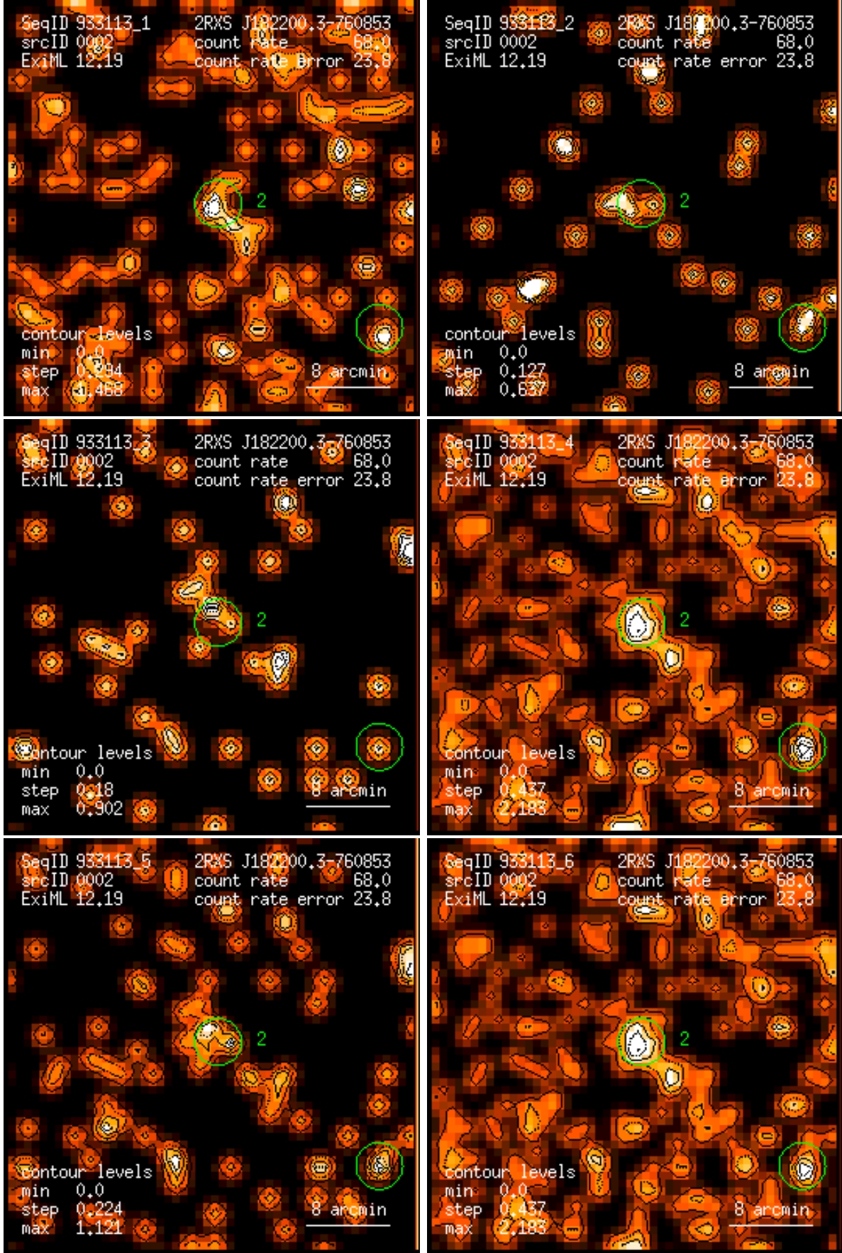
Figure 2: RASS 933113: detection 0002: band rate images, Gaussian filter: (1) PSPC channels 11 – 41, (2) 52 – 90, (3) 91 – 201, (4) 11 – 235, (5) 52 – 201, (6) 11 – 201. Broad band rates in counts/ks. Band rate contour levels in counts/ks/arcmin 2 .
