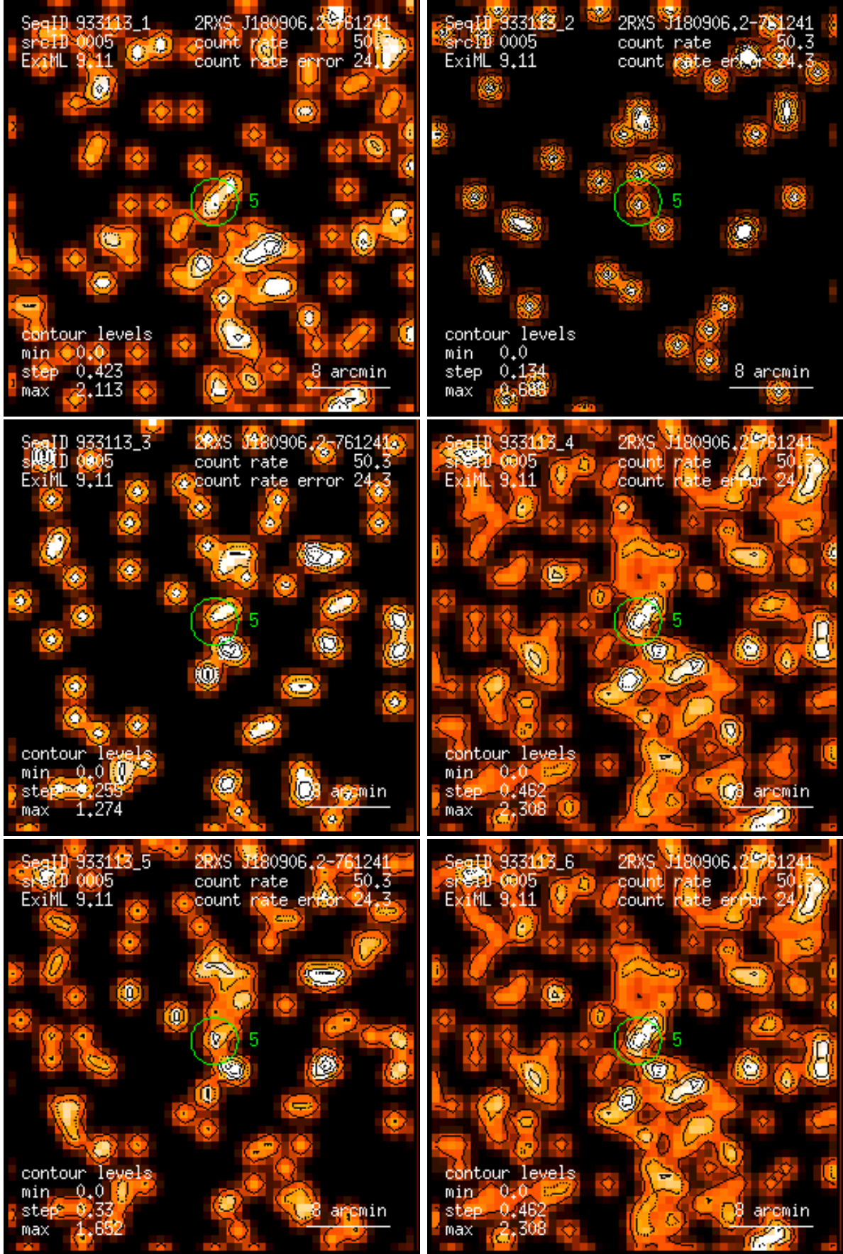
Figure 5: RASS 933113: detection 0005: band rate images, Gaussian filter: (1) PSPC channels 11 – 41, (2) 52 – 90, (3) 91 – 201, (4) 11 – 235, (5) 52 – 201, (6) 11 – 201. Broad band rates in counts/ks. Band rate contour levels in counts/ks/arcmin 2 .
