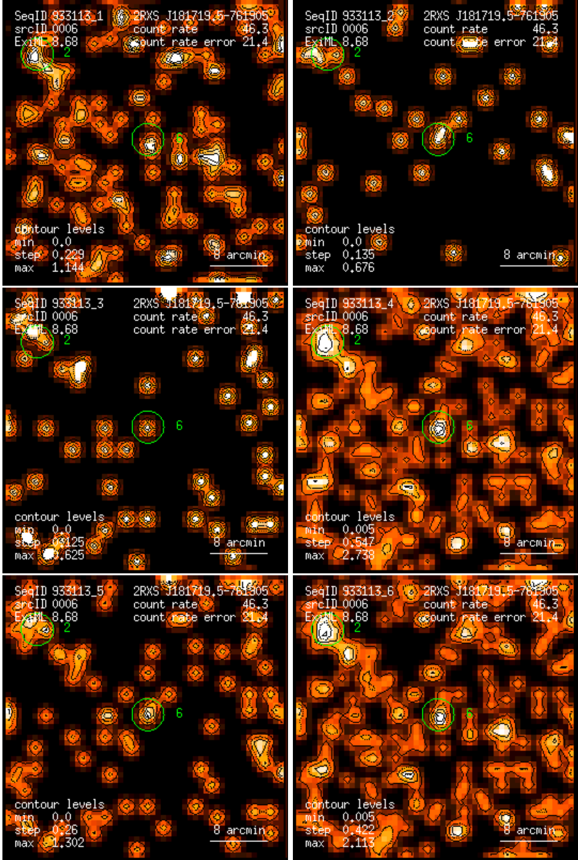
Figure 6: RASS 933113: detection 0006: band rate images, Gaussian filter: (1) PSPC channels 11 – 41, (2) 52 – 90, (3) 91 – 201, (4) 11 – 235, (5) 52 – 201, (6) 11 – 201. Broad band rates in counts/ks. Band rate contour levels in counts/ks/arcmin 2 .
