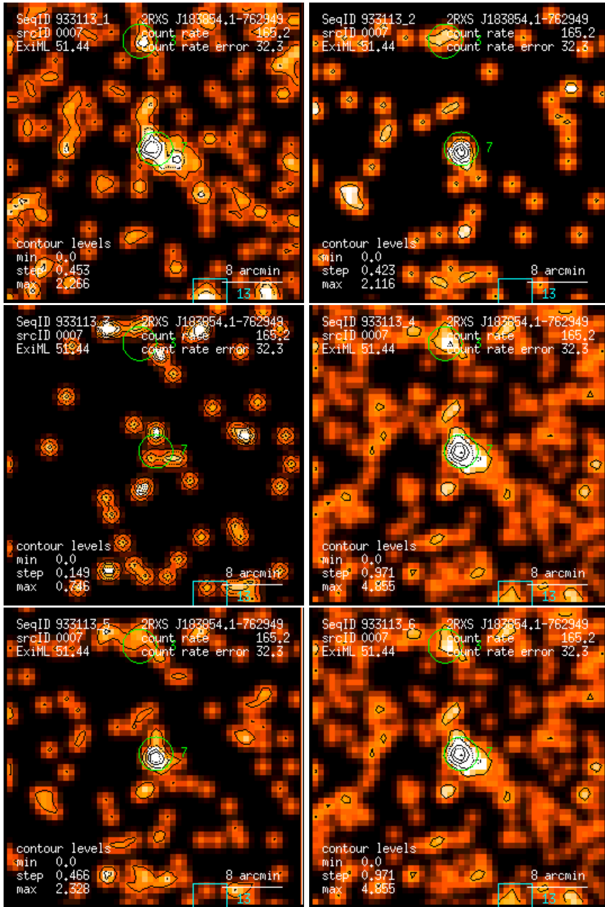
Figure 7: RASS 933113: detection 0007: band rate images, Gaussian filter: (1) PSPC channels 11 – 41, (2) 52 – 90, (3) 91 – 201, (4) 11 – 235, (5) 52 – 201, (6) 11 – 201. Broad band rates in counts/ks. Band rate contour levels in counts/ks/arcmin 2 .
