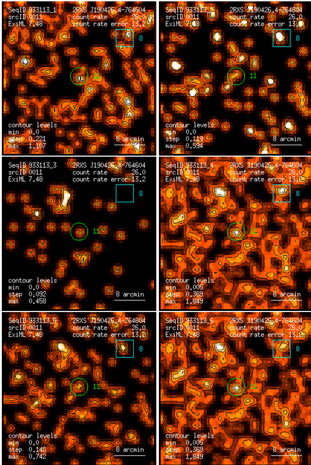
Figure 11: RASS 933113: detection 0011: band rate images, Gaussian filter: (1) PSPC channels 11 – 41, (2) 52 – 90, (3) 91 – 201, (4) 11 – 235, (5) 52 – 201, (6) 11 – 201. Broad band rates in counts/ks. Band rate contour levels in counts/ks/arcmin 2 .
