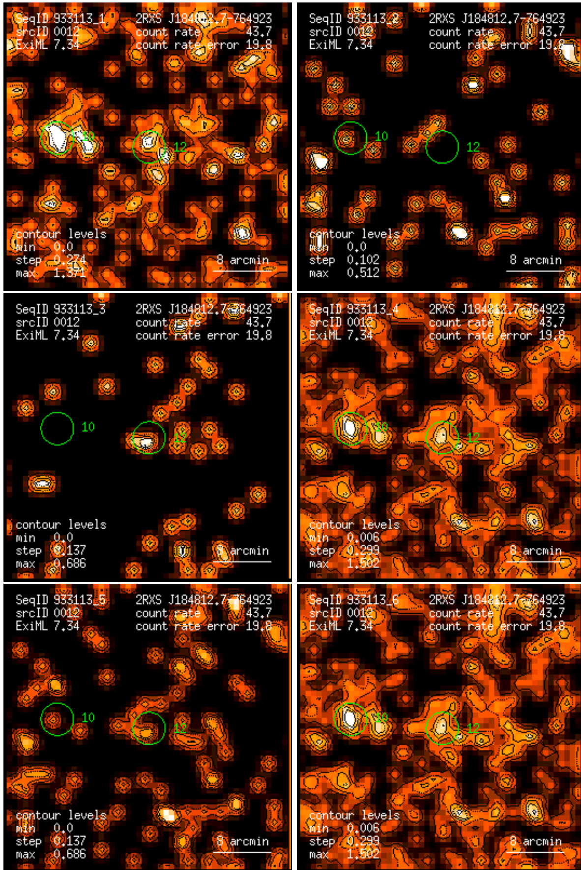
Figure 12: RASS 933113: detection 0012: band rate images, Gaussian filter: (1) PSPC channels 11 – 41, (2) 52 – 90, (3) 91 – 201, (4) 11 – 235, (5) 52 – 201, (6) 11 – 201. Broad band rates in counts/ks. Band rate contour levels in counts/ks/arcmin 2 .
