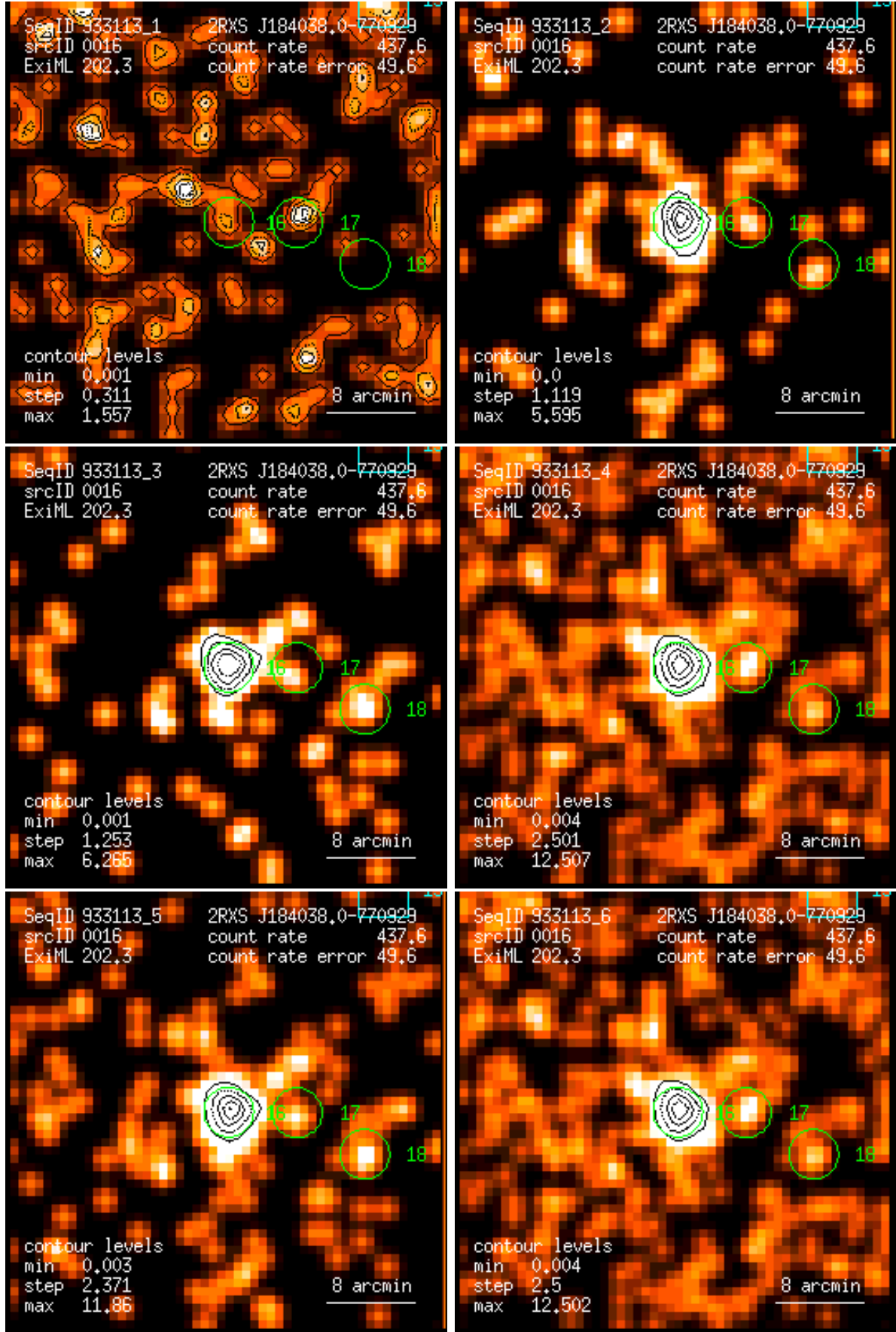
Figure 16: RASS 933113: detection 0016: band rate images, Gaussian filter: (1) PSPC channels 11 – 41, (2) 52 – 90, (3) 91 – 201, (4) 11 – 235, (5) 52 – 201, (6) 11 – 201. Broad band rates in counts/ks. Band rate contour levels in counts/ks/arcmin 2 .
