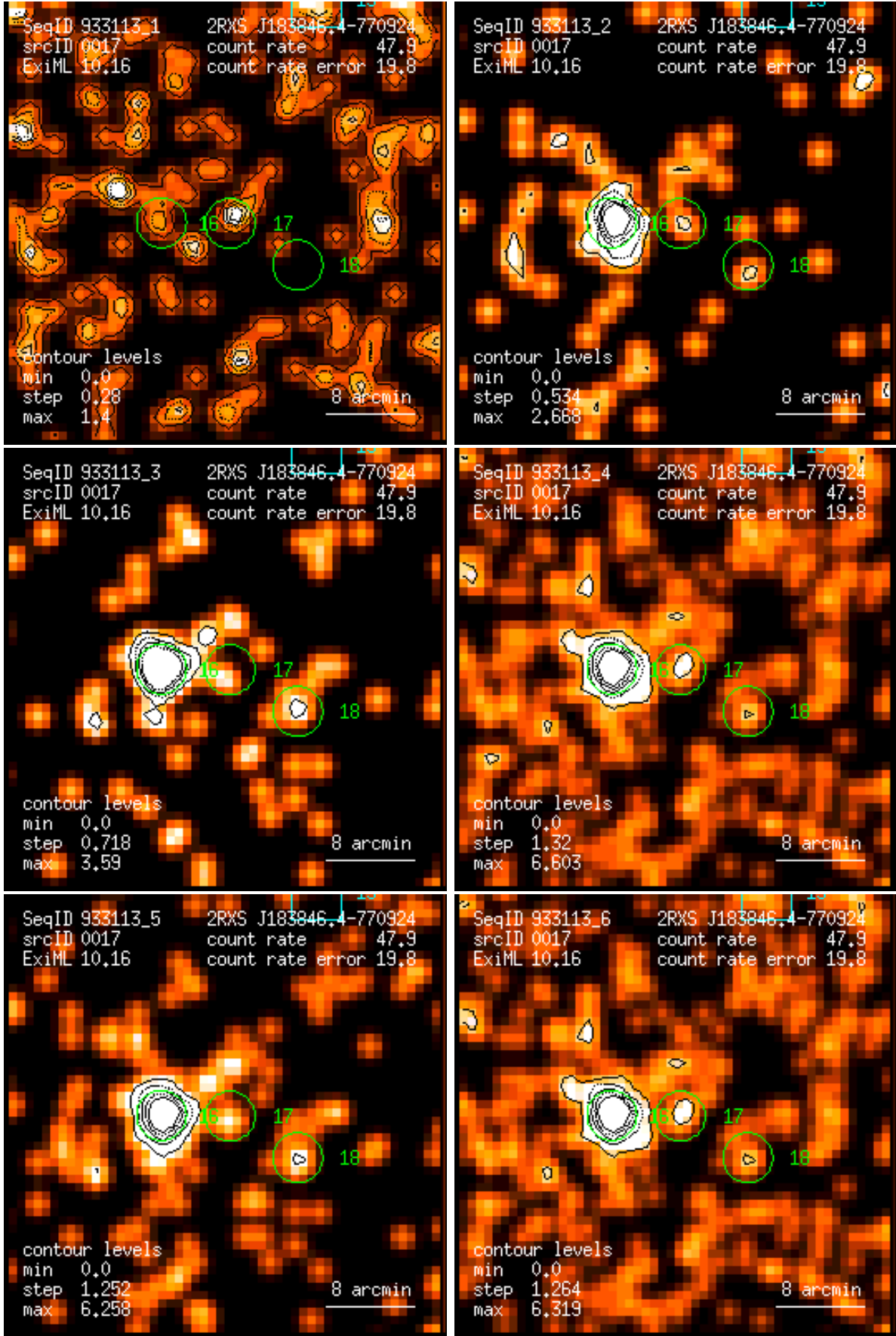
Figure 17: RASS 933113: detection 0017: band rate images, Gaussian filter: (1) PSPC channels 11 – 41, (2) 52 – 90, (3) 91 – 201, (4) 11 – 235, (5) 52 – 201, (6) 11 – 201. Broad band rates in counts/ks. Band rate contour levels in counts/ks/arcmin 2 .
