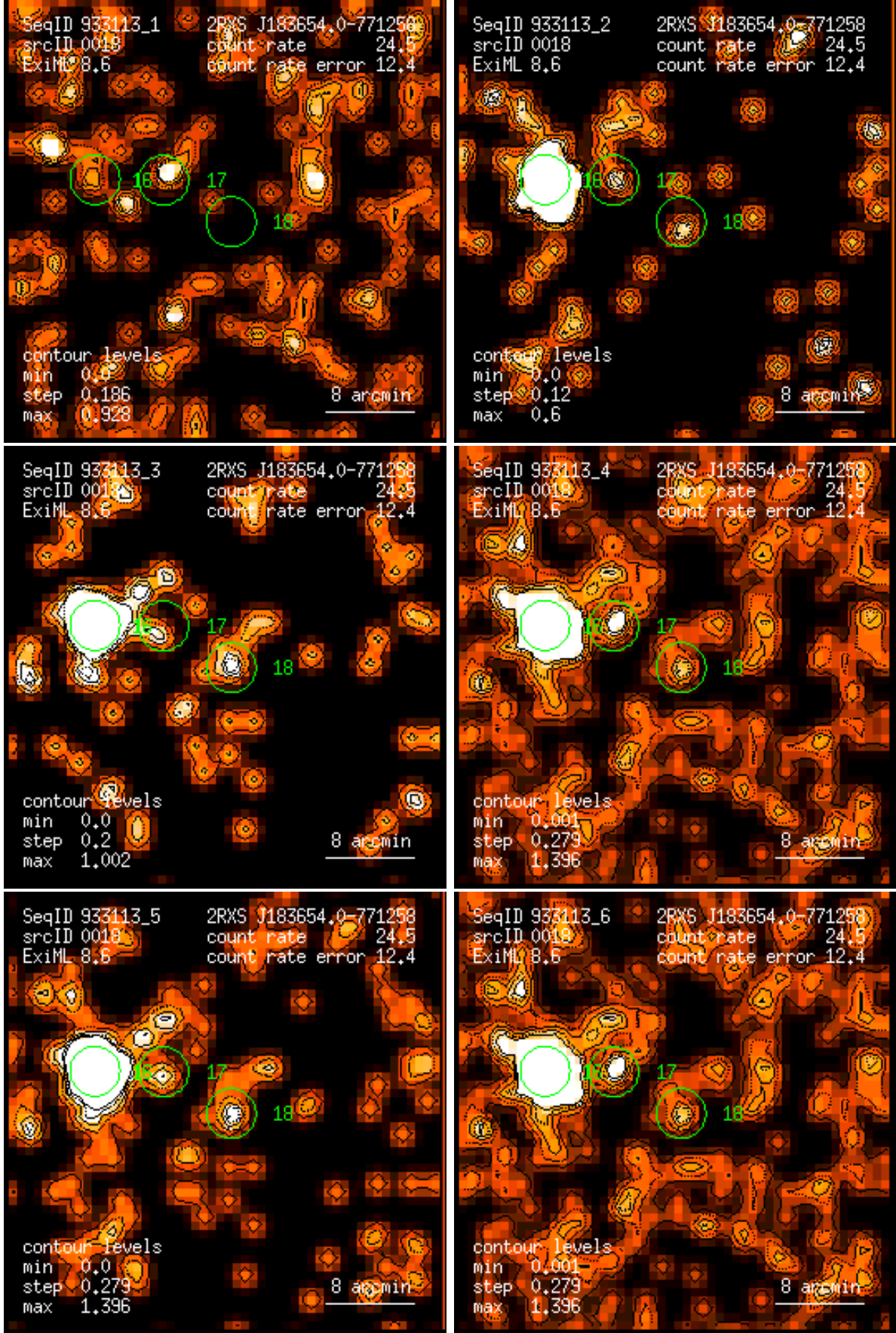
Figure 18: RASS 933113: detection 0018: band rate images, Gaussian filter: (1) PSPC channels 11 – 41, (2) 52 – 90, (3) 91 – 201, (4) 11 – 235, (5) 52 – 201, (6) 11 – 201. Broad band rates in counts/ks. Band rate contour levels in counts/ks/arcmin 2 .
