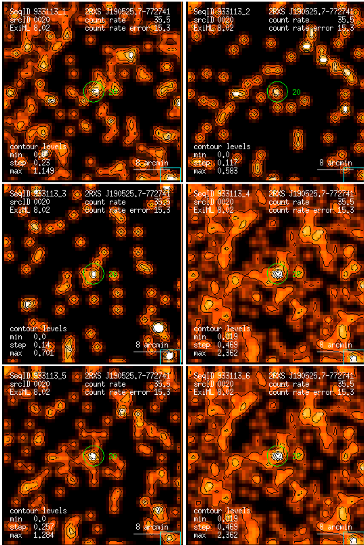
Figure 20: RASS 933113: detection 0020: band rate images, Gaussian filter: (1) PSPC channels 11 – 41, (2) 52 – 90, (3) 91 – 201, (4) 11 – 235, (5) 52 – 201, (6) 11 – 201. Broad band rates in counts/ks. Band rate contour levels in counts/ks/arcmin 2 .
