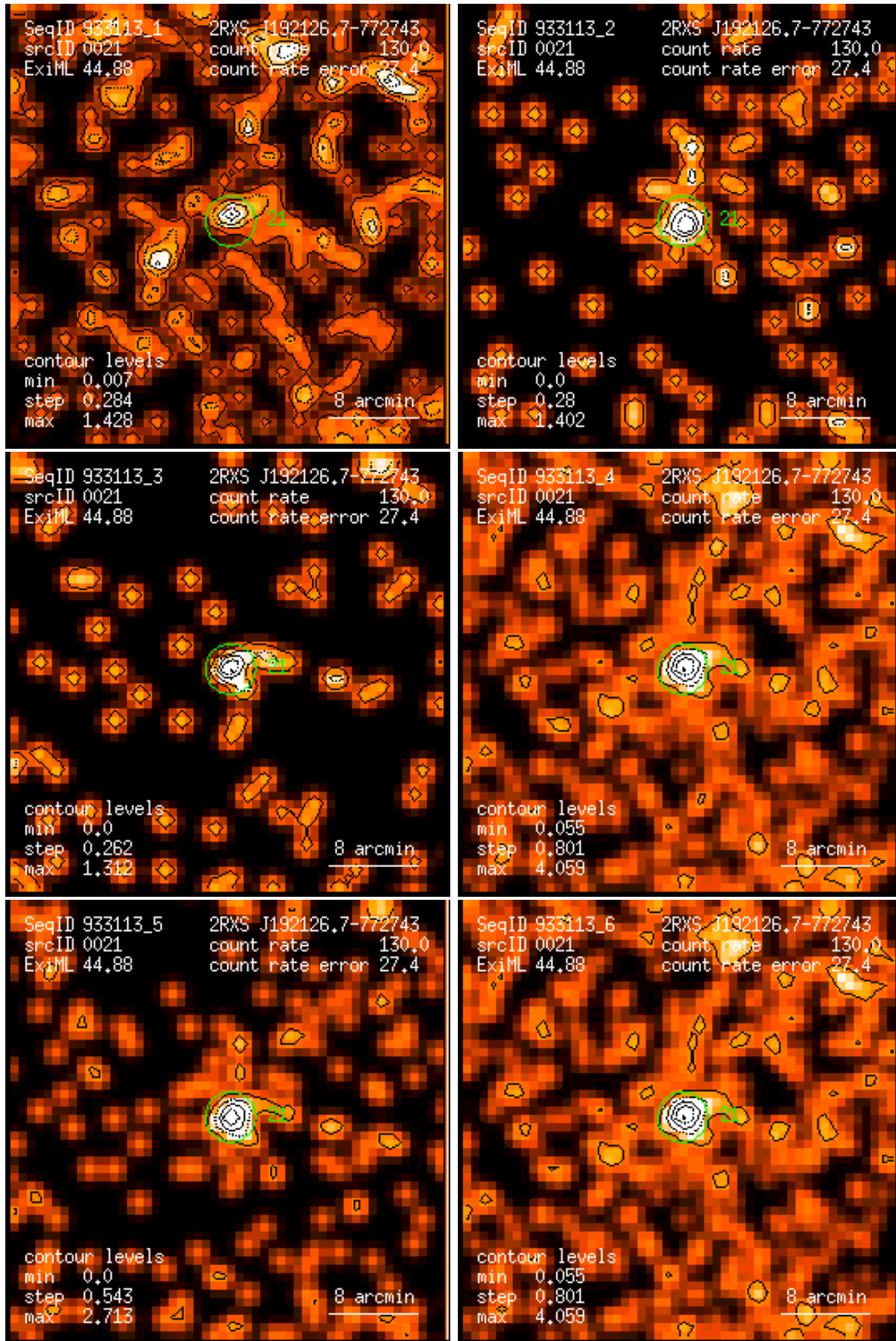
Figure 21: RASS 933113: detection 0021: band rate images, Gaussian filter: (1) PSPC channels 11 – 41, (2) 52 – 90, (3) 91 – 201, (4) 11 – 235, (5) 52 – 201, (6) 11 – 201. Broad band rates in counts/ks. Band rate contour levels in counts/ks/arcmin 2 .
