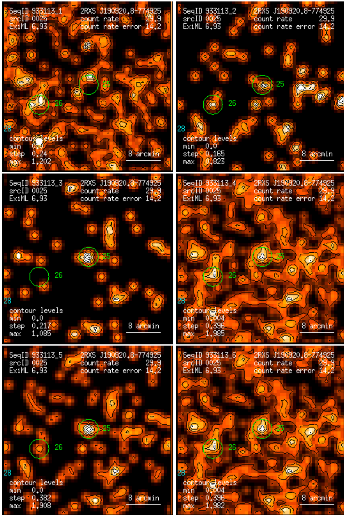
Figure 25: RASS 933113: detection 0025: band rate images, Gaussian filter: (1) PSPC channels 11 – 41, (2) 52 – 90, (3) 91 – 201, (4) 11 – 235, (5) 52 – 201, (6) 11 – 201. Broad band rates in counts/ks. Band rate contour levels in counts/ks/arcmin 2 .
