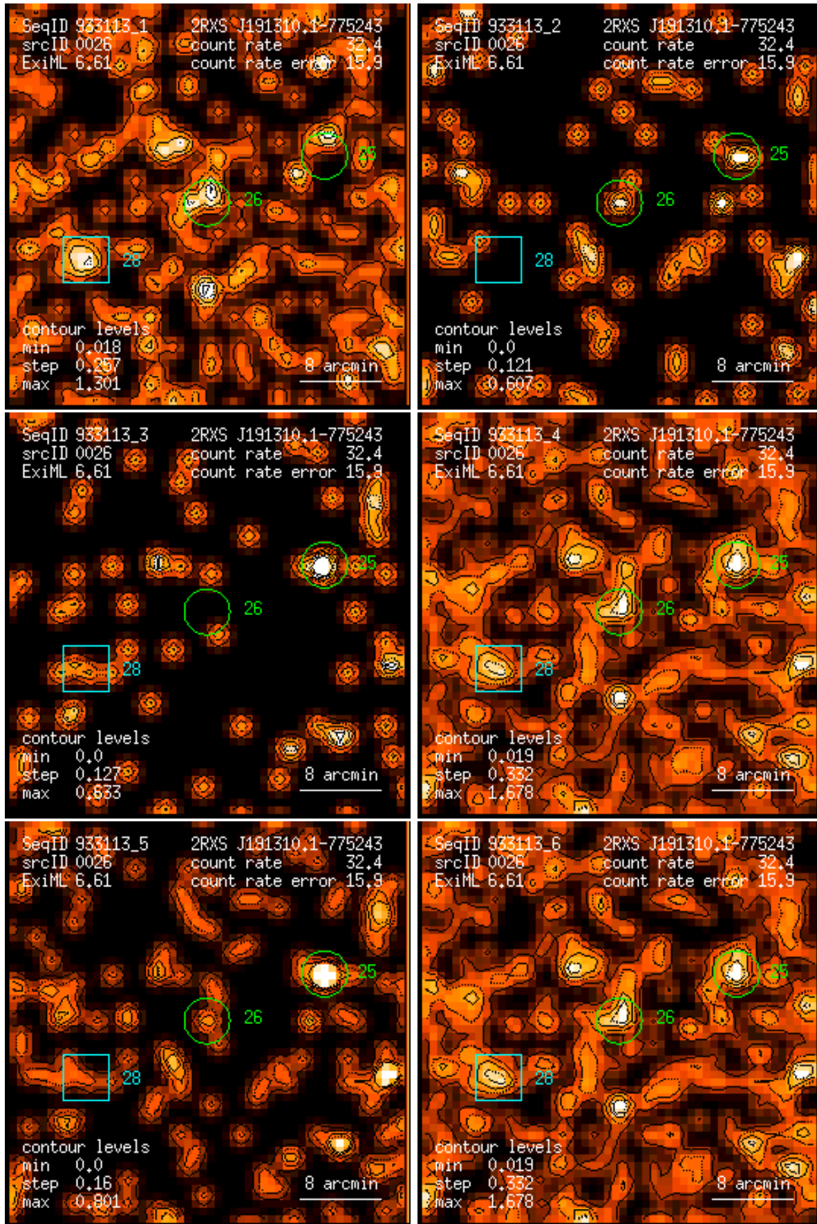
Figure 26: RASS 933113: detection 0026: band rate images, Gaussian filter: (1) PSPC channels 11 – 41, (2) 52 – 90, (3) 91 – 201, (4) 11 – 235, (5) 52 – 201, (6) 11 – 201. Broad band rates in counts/ks. Band rate contour levels in counts/ks/arcmin 2 .
