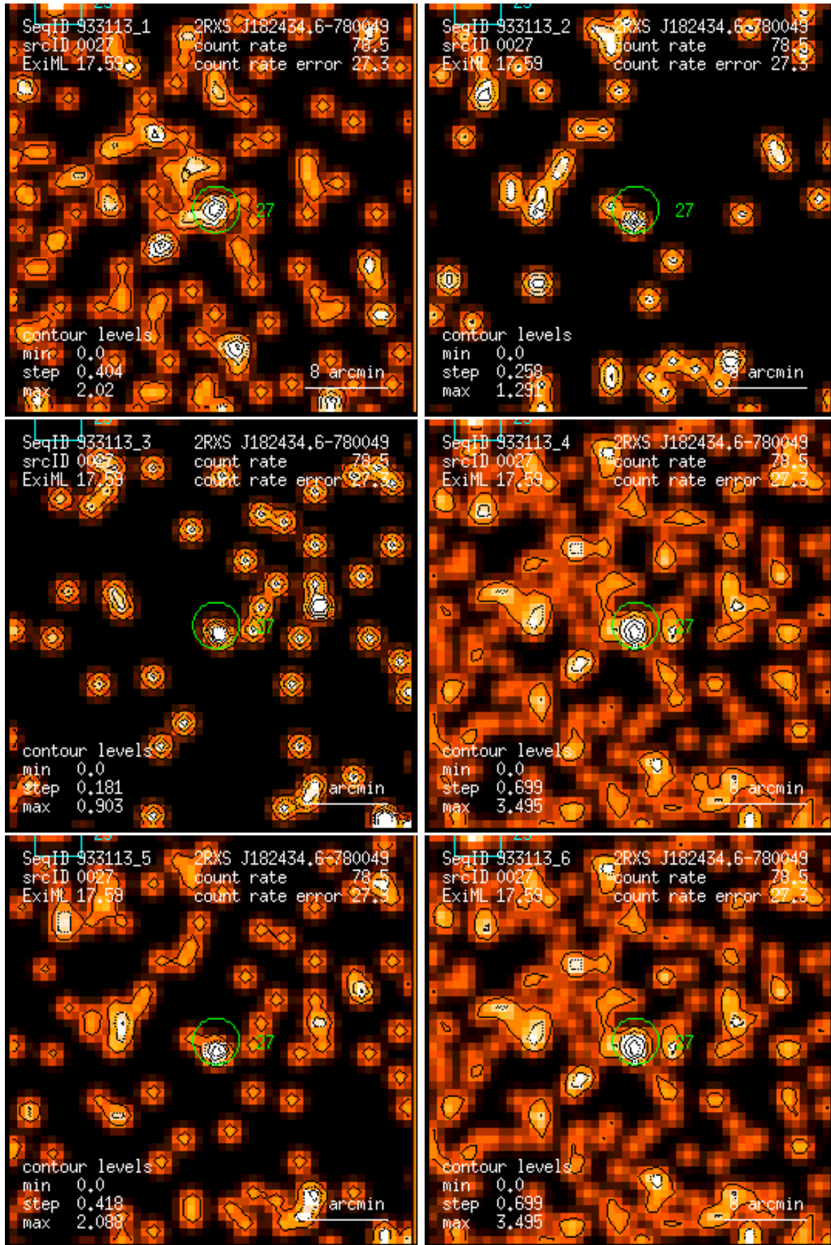
Figure 27: RASS 933113: detection 0027: band rate images, Gaussian filter: (1) PSPC channels 11 – 41, (2) 52 – 90, (3) 91 – 201, (4) 11 – 235, (5) 52 – 201, (6) 11 – 201. Broad band rates in counts/ks. Band rate contour levels in counts/ks/arcmin 2 .
