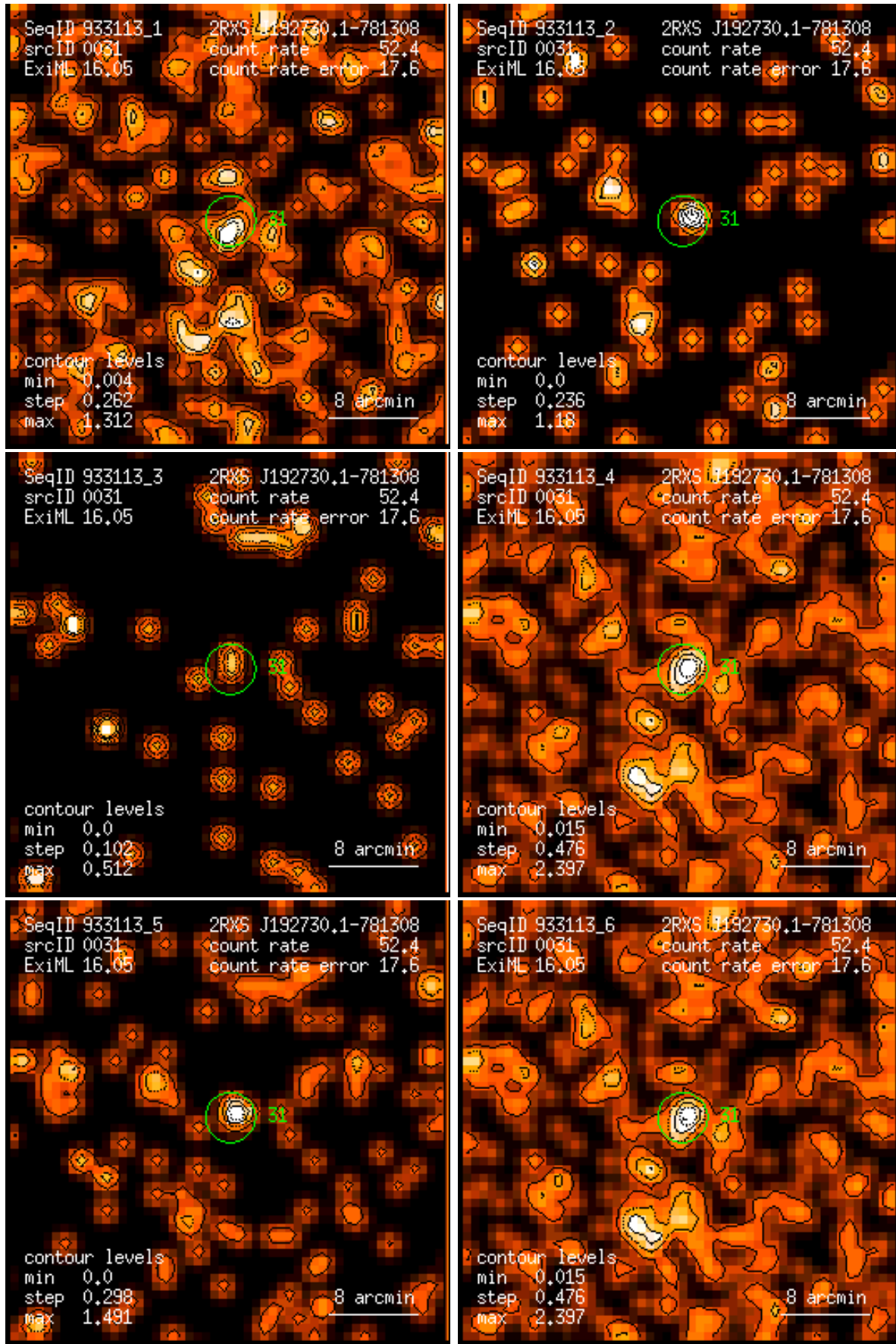
Figure 31: RASS 933113: detection 0031: band rate images, Gaussian filter: (1) PSPC channels 11 – 41, (2) 52 – 90, (3) 91 – 201, (4) 11 – 235, (5) 52 – 201, (6) 11 – 201. Broad band rates in counts/ks. Band rate contour levels in counts/ks/arcmin 2 .
