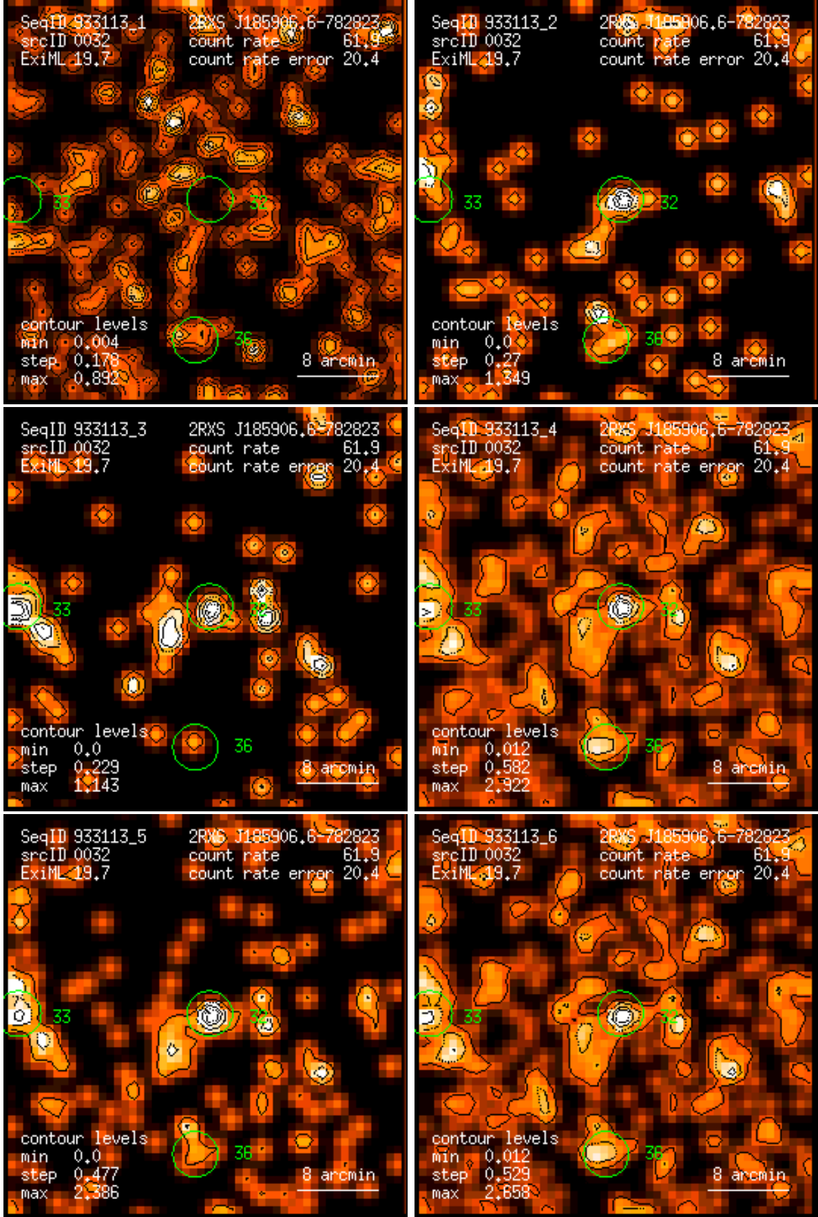
Figure 32: RASS 933113: detection 0032: band rate images, Gaussian filter: (1) PSPC channels 11 – 41, (2) 52 – 90, (3) 91 – 201, (4) 11 – 235, (5) 52 – 201, (6) 11 – 201. Broad band rates in counts/ks. Band rate contour levels in counts/ks/arcmin 2 .
