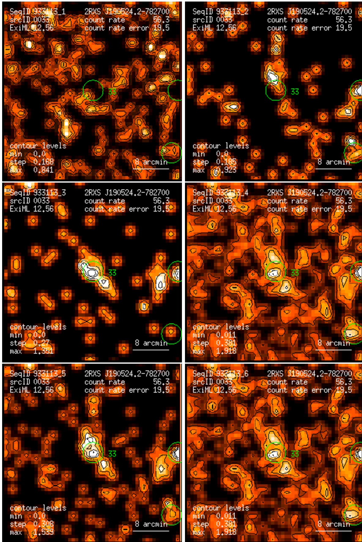
Figure 33: RASS 933113: detection 0033: band rate images, Gaussian filter: (1) PSPC channels 11 – 41, (2) 52 – 90, (3) 91 – 201, (4) 11 – 235, (5) 52 – 201, (6) 11 – 201. Broad band rates in counts/ks. Band rate contour levels in counts/ks/arcmin 2 .
